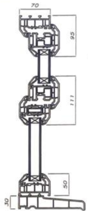
Section D - D
