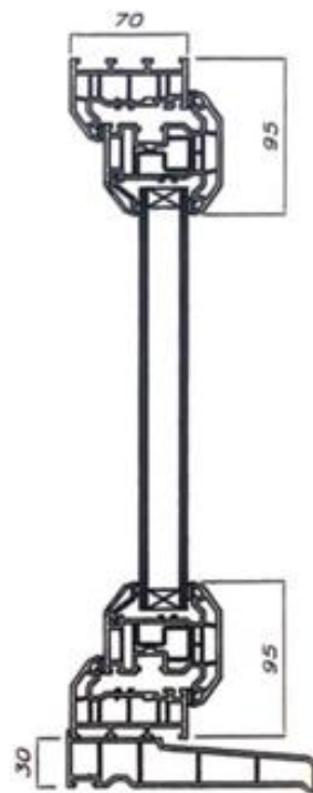
Section C - C
