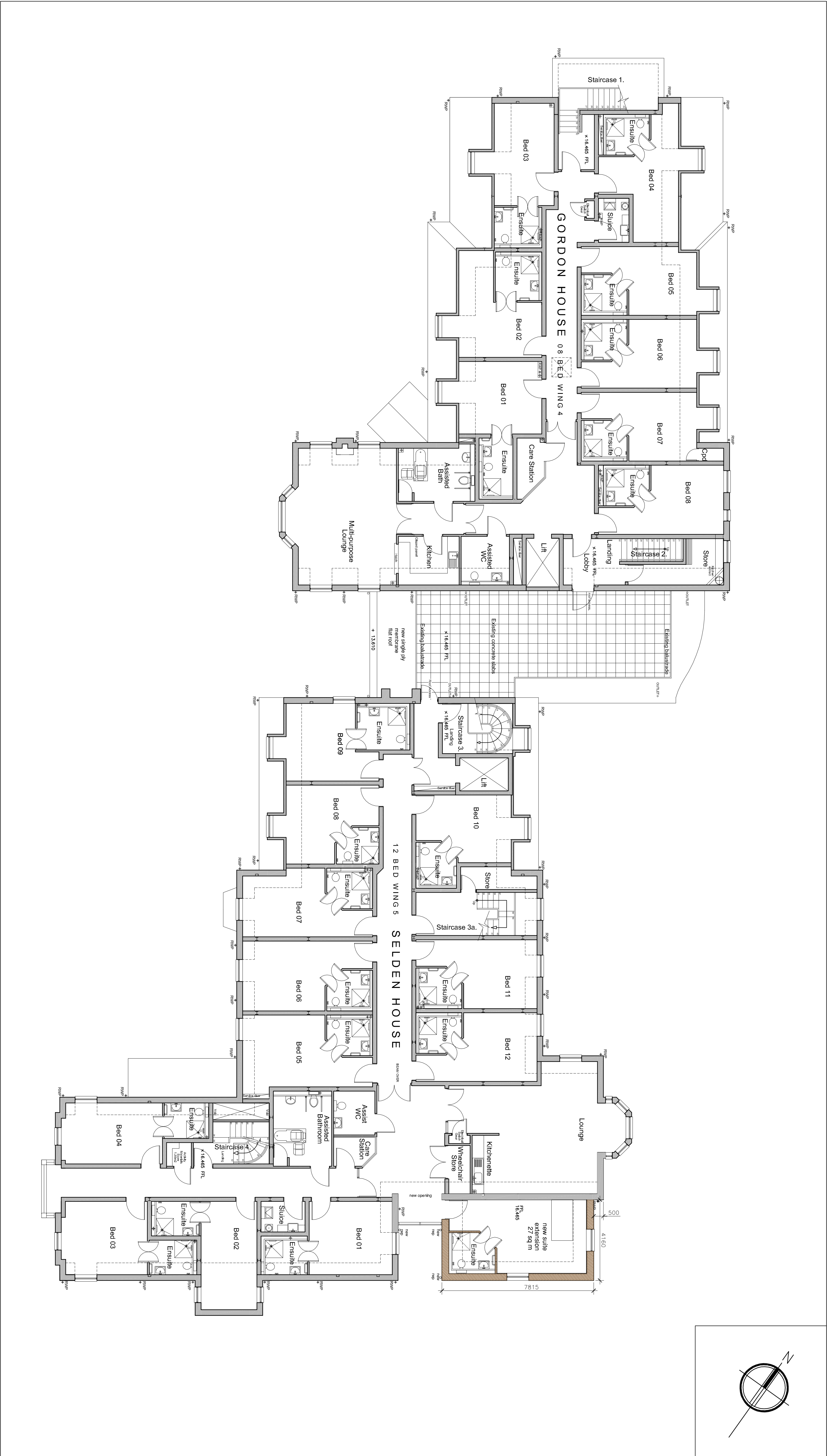
1:100 Second Floor Plan as Proposed
