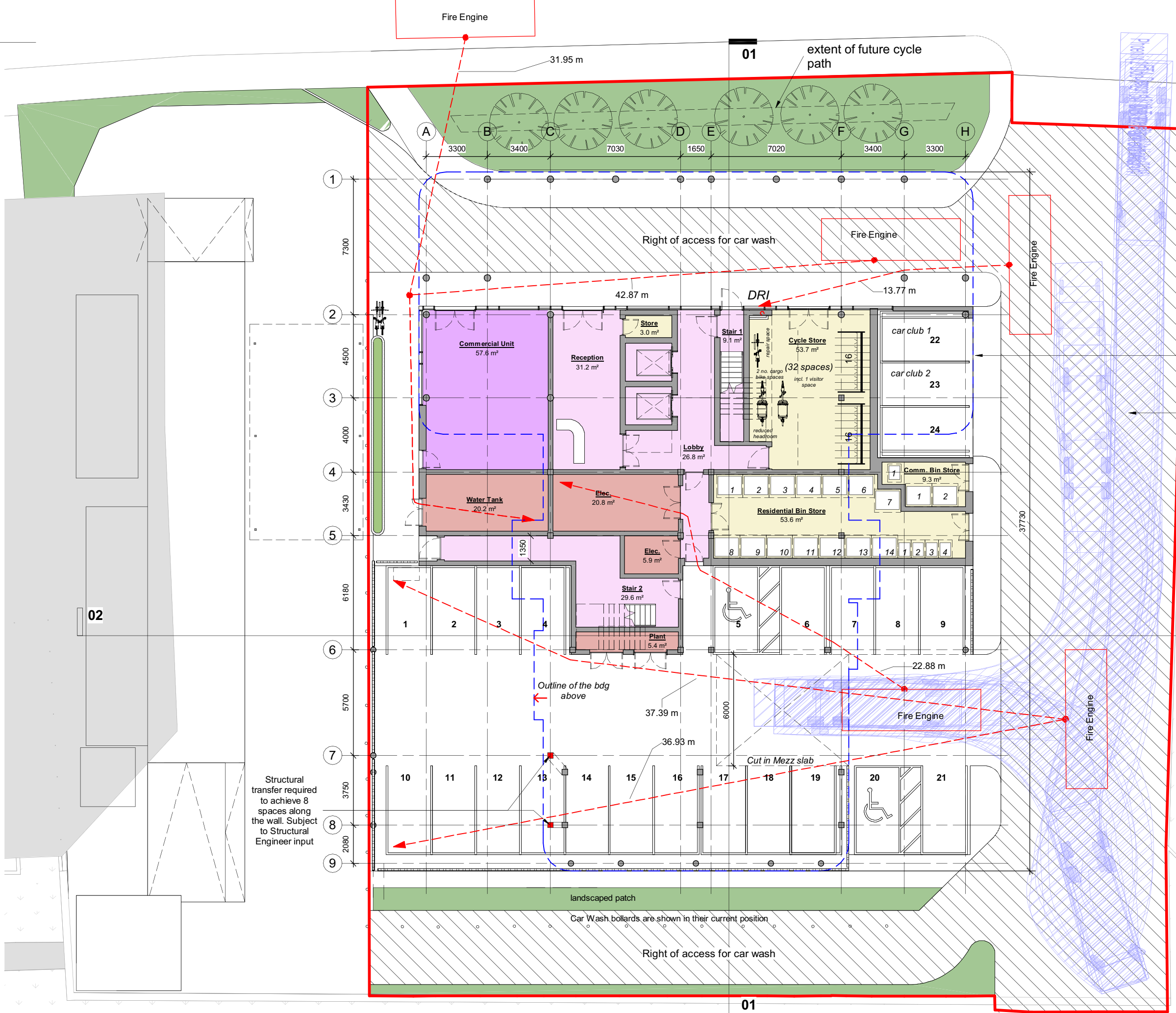
1 Ground Floor Fire Hose Distance 1 : 200
