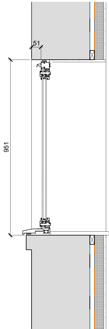
Window Section 1:10
