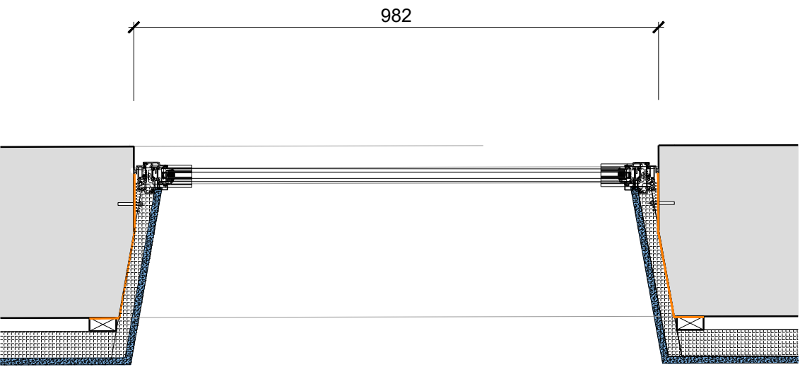
Window Plan 1:10
