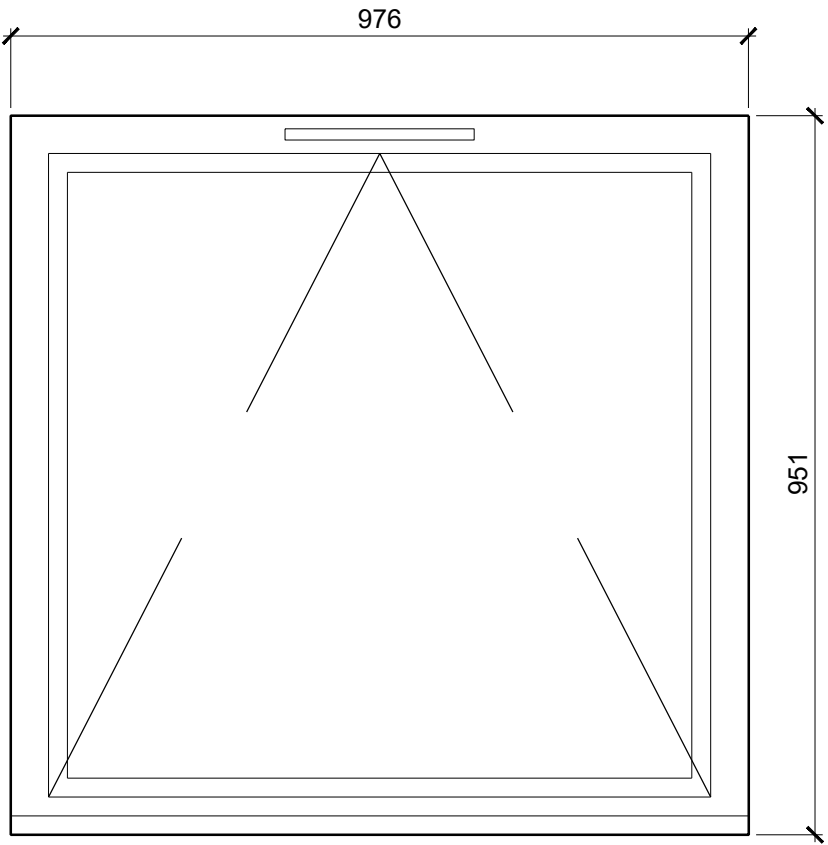
External Window Elevation 1:10
