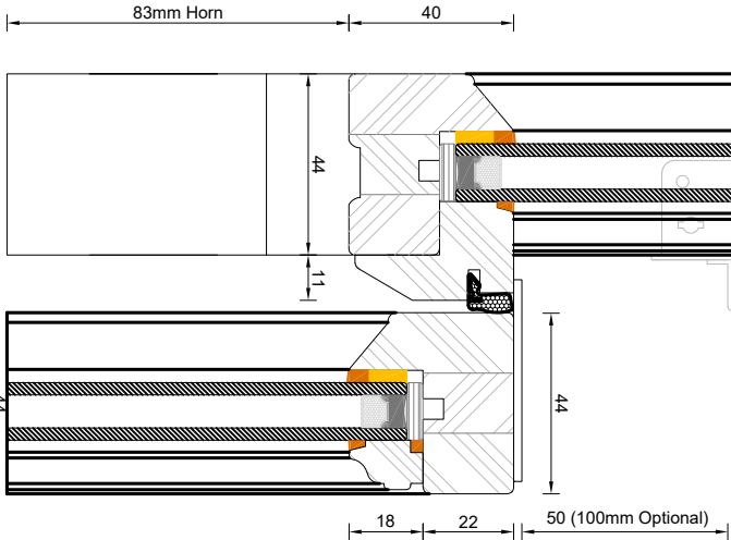
Proposed Meeting Rail Section @ 1 : 2
