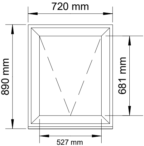
Toilet Window (Proposed) (Obscured Glass)
