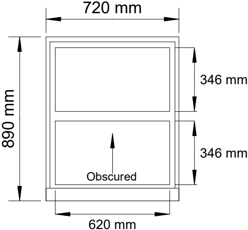
Toilet Window (Existing) (Part Obscured Glass)
