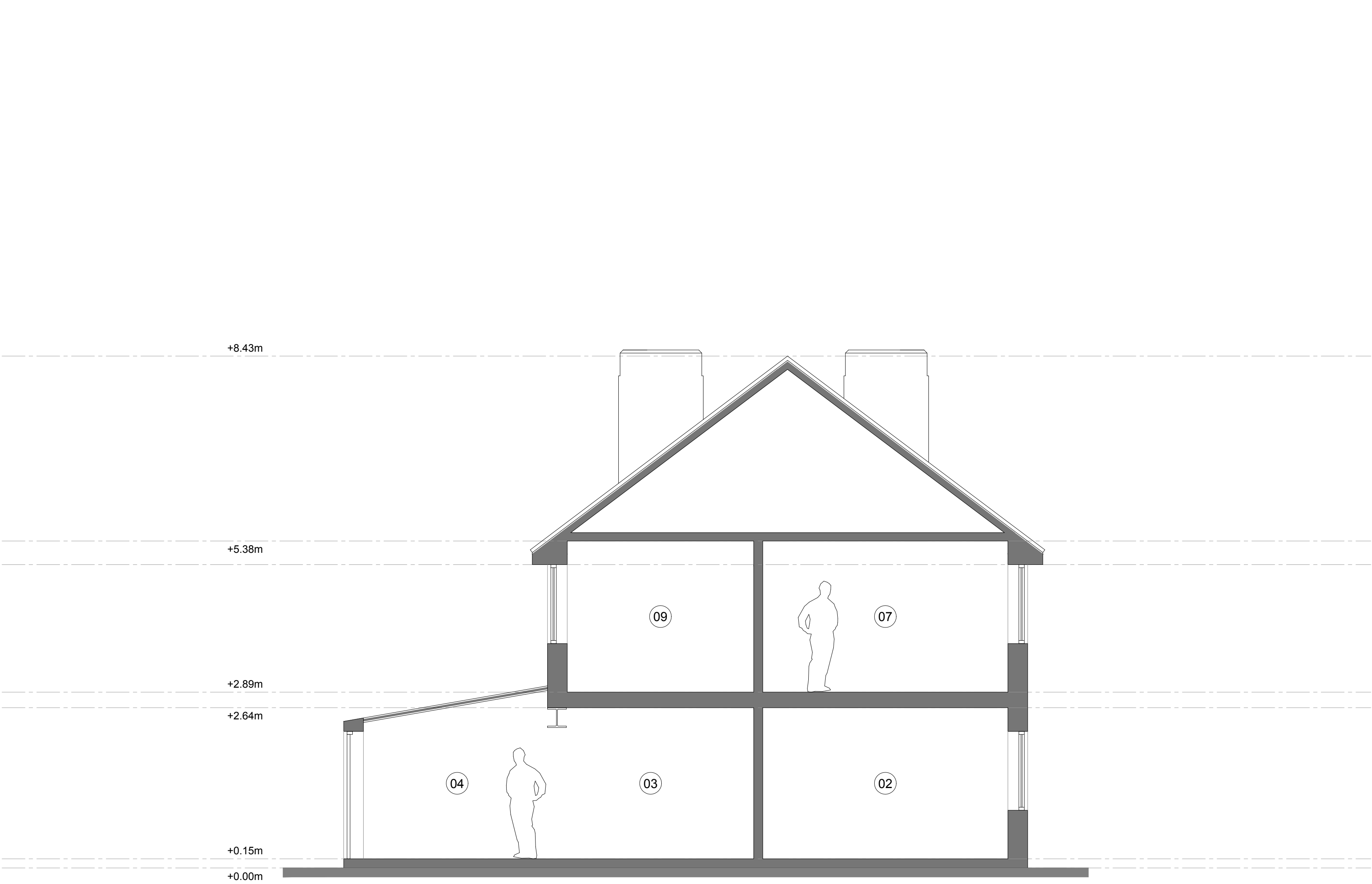
SECTION A - A
