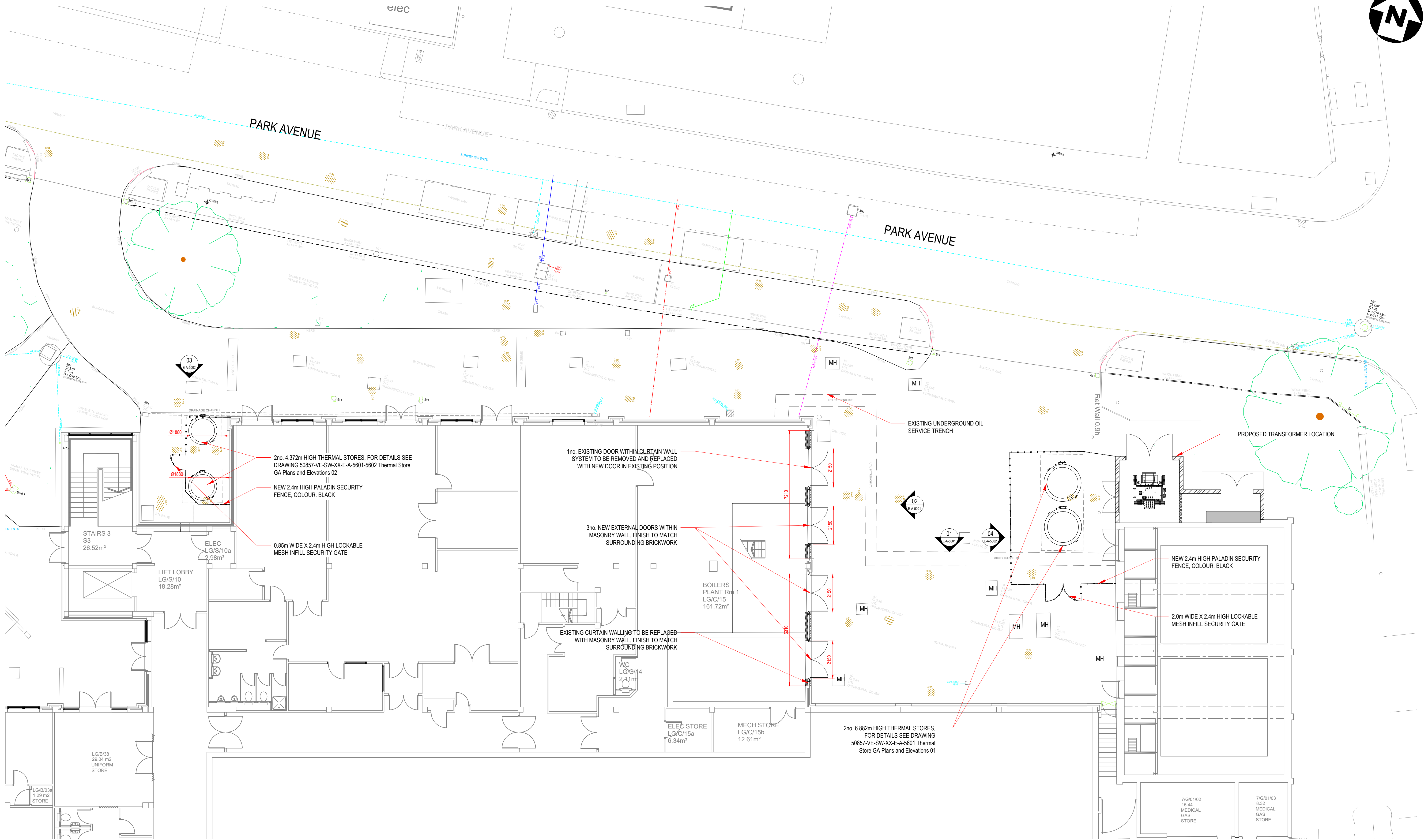
PROPOSED SITE PLAN (1:100 SCALE)
