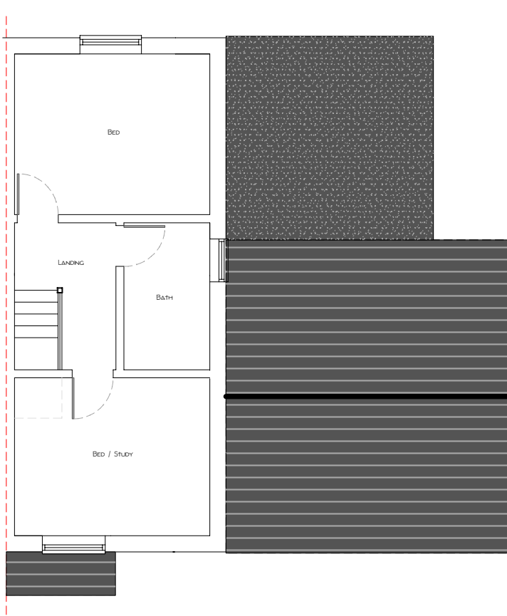
1st FLOOR EXISTING LAYOUT 100001
