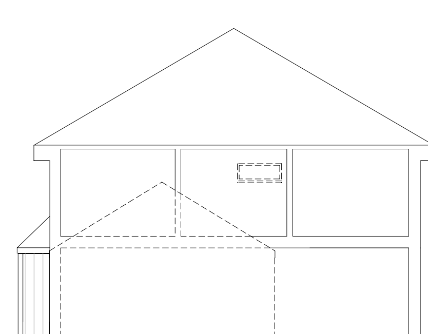
SIDE SECTION / NORTH EXISTING ELEVATION 100001
