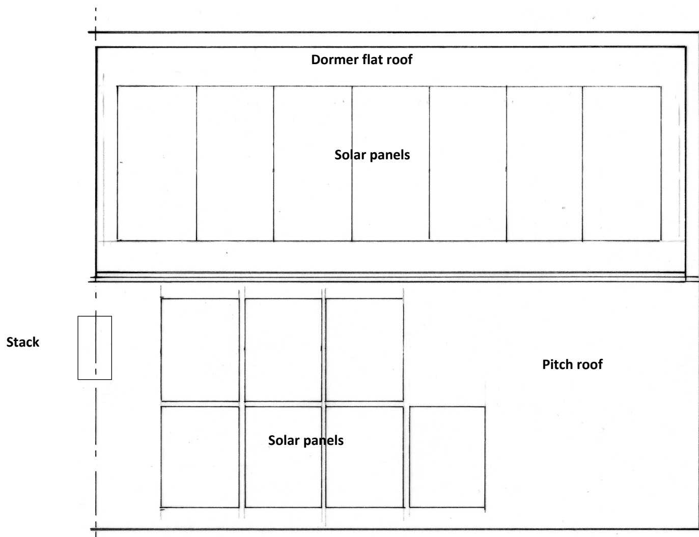
Proposed Roof Plan 1:50
