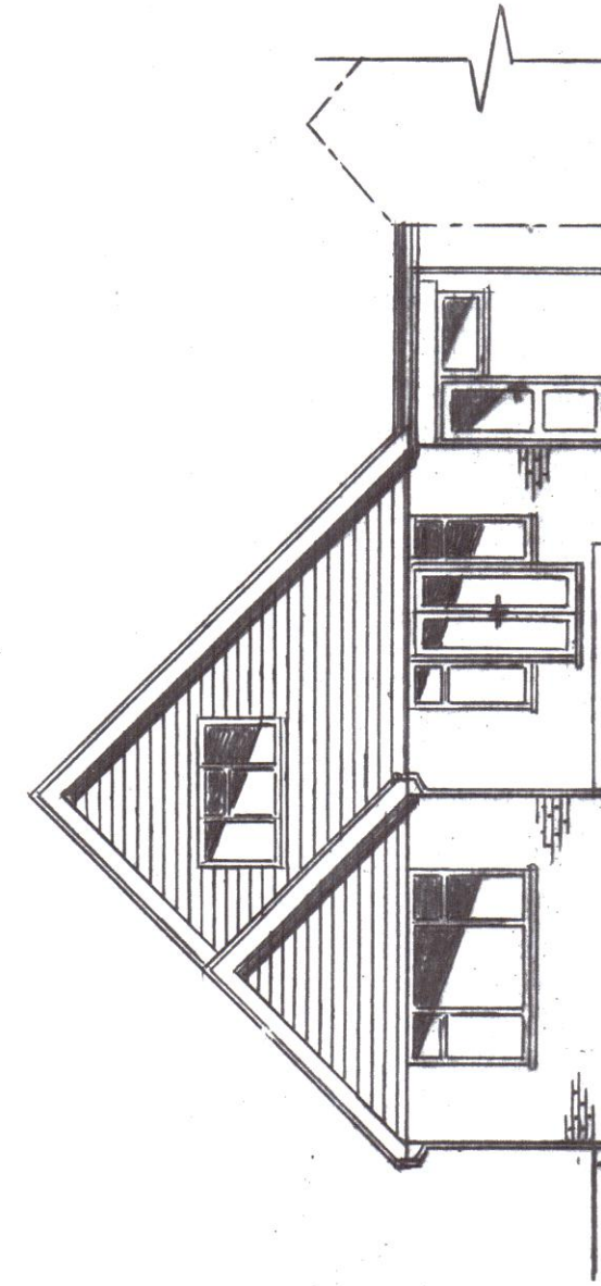
REAR/WEST ELEVATION 1:100
