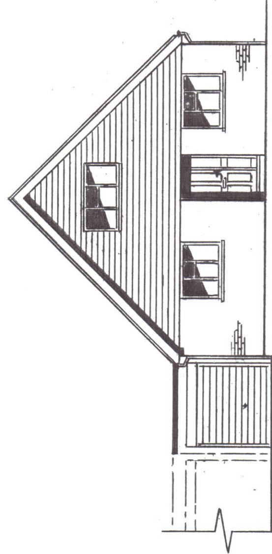
FRONT/EAST ELEVATION 1:100
