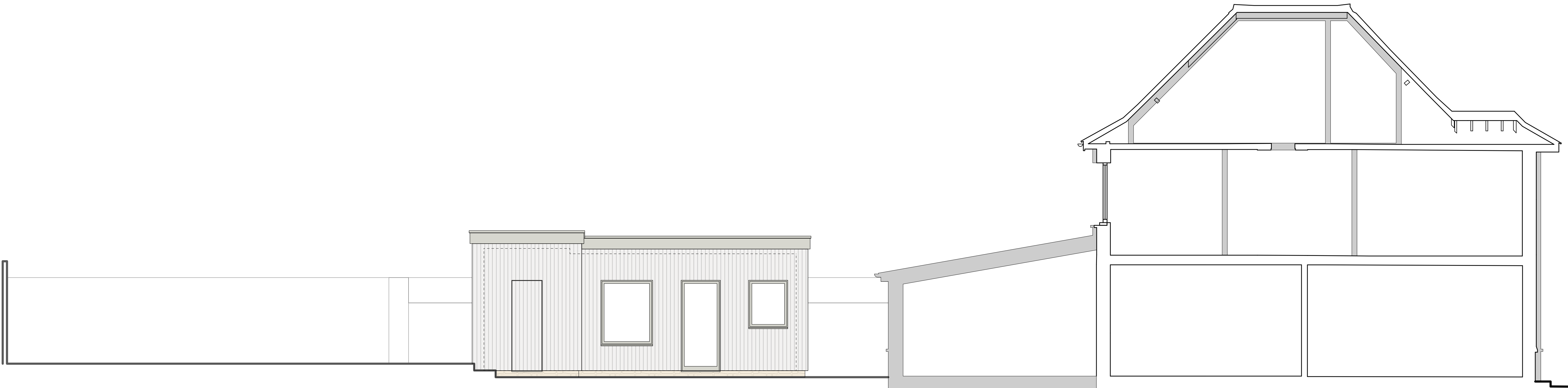
017.2 Section- Proposed Scale: 1:50
