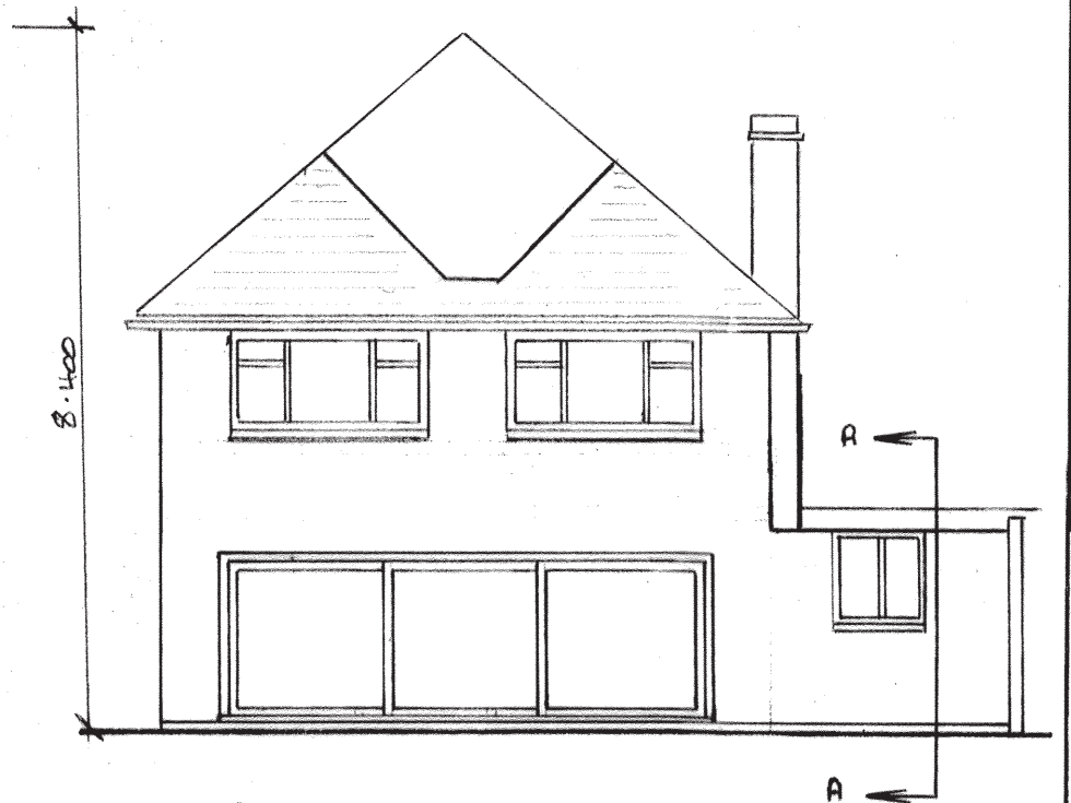
PROPOSED REAR ELEVATION (NORTH)
