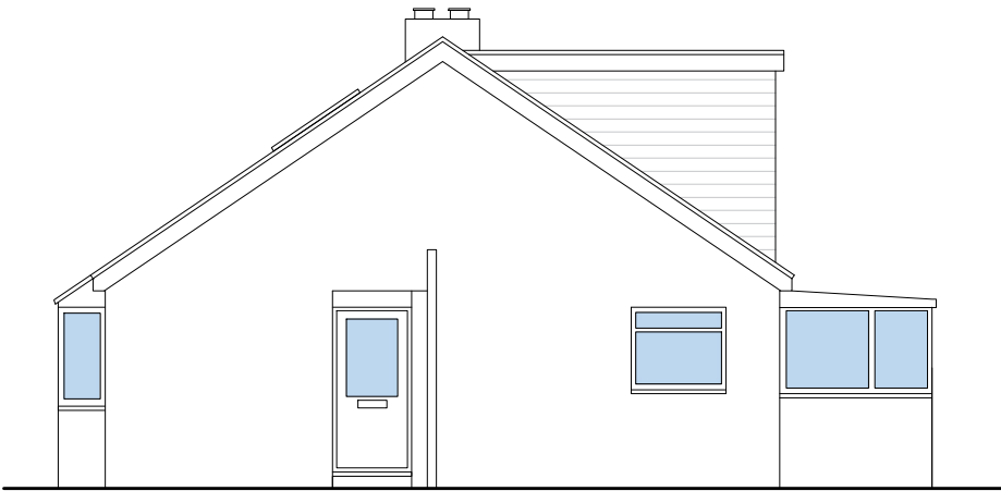
EXISTING SIDE ELEVATION (N) 1:100
