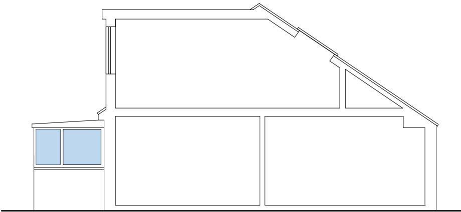
EXISTING SIDE SECTION/ELEVATION (S) 1:100
