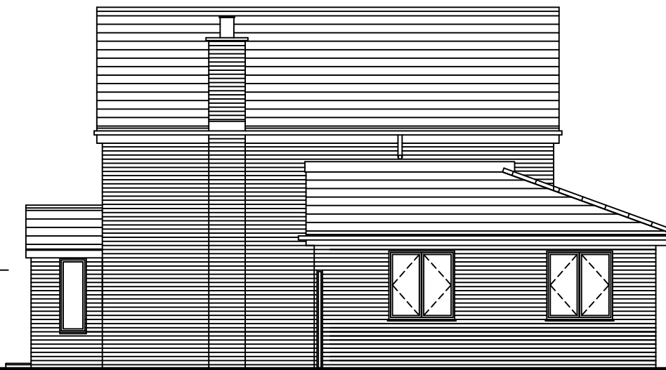
EXISTING SIDE ELEVATION - NORTH
