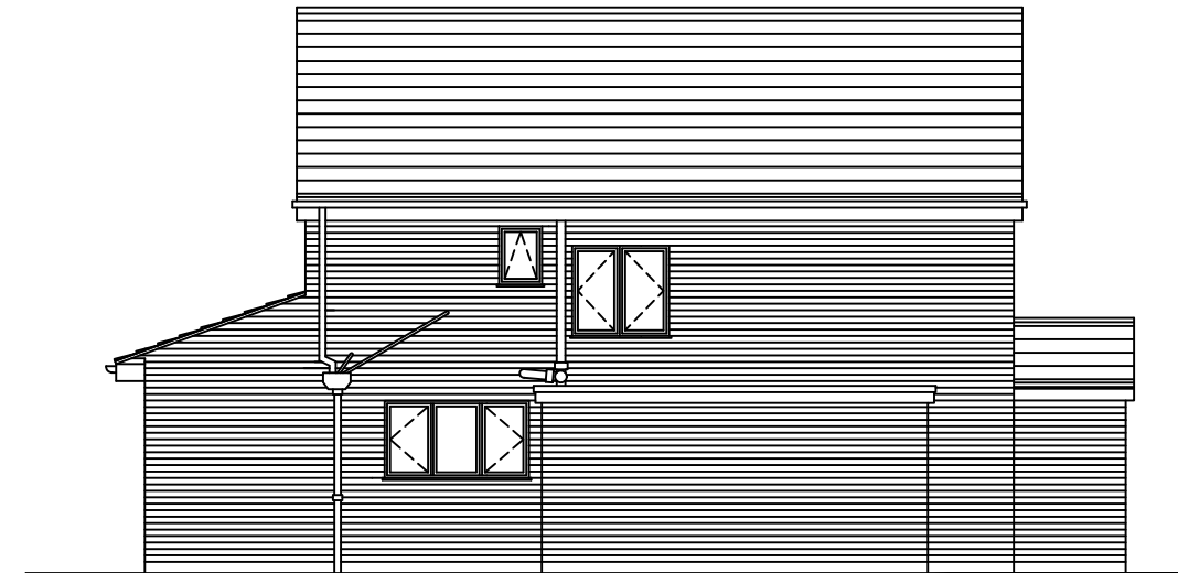
EXISTING SIDE ELEVATION - SOUTH
