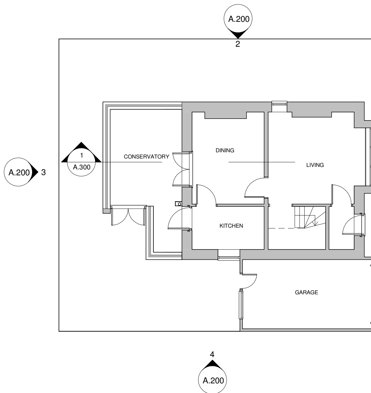
1 GROUND FLOOR 1 : 100
