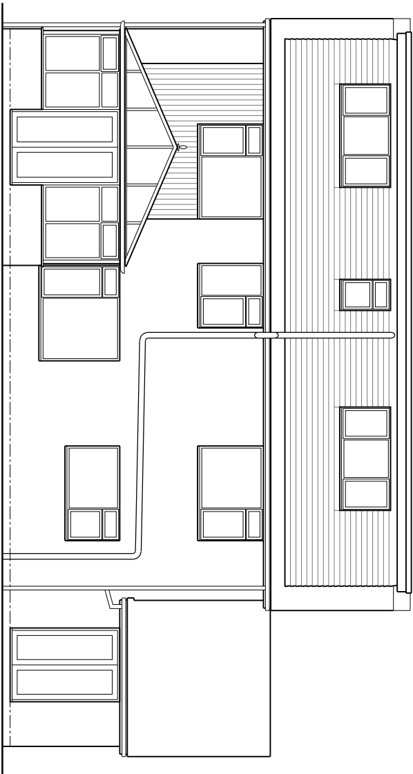
Existing Rear (SE) Elevation 1:100
