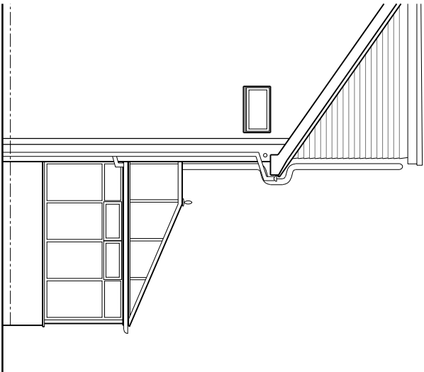
Existing Side (SW) Elevation 1:100
