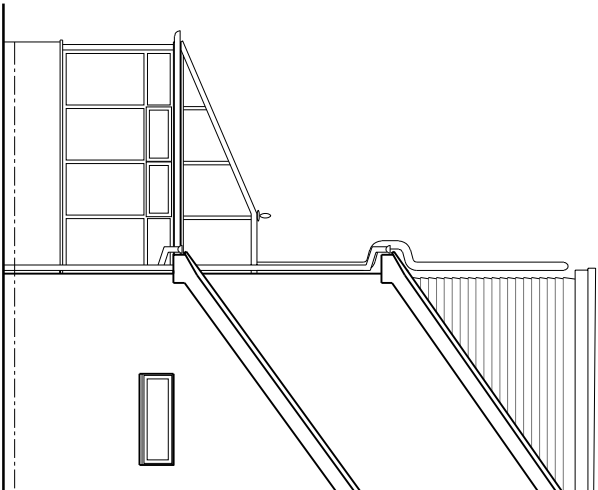
Existing Side (NE) Elevation 1:100
