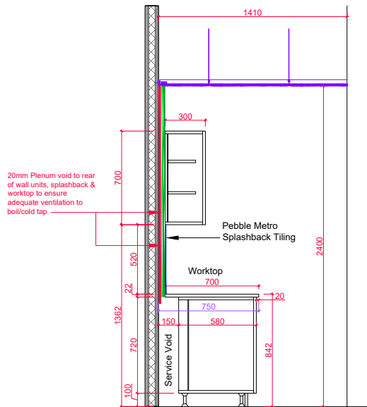
Kitchen Side Section A-A
