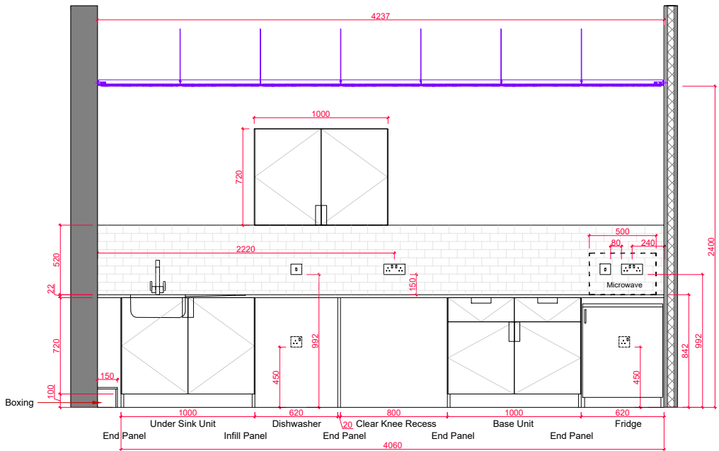
Kitchen Front Elevation
