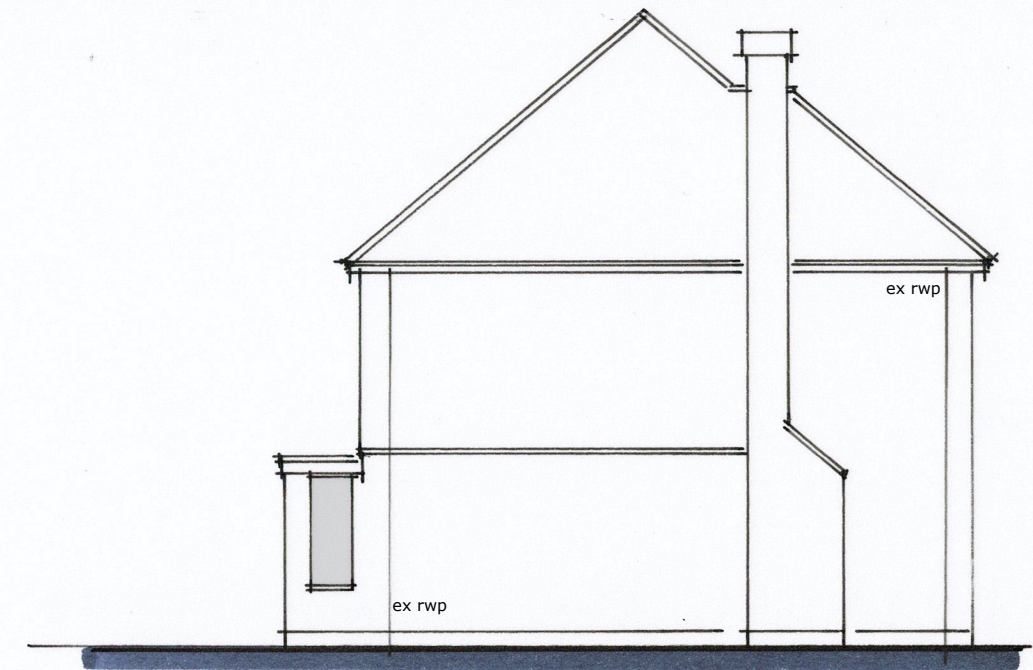
SIDE (n) ELEVATION 1:100 @ A3
