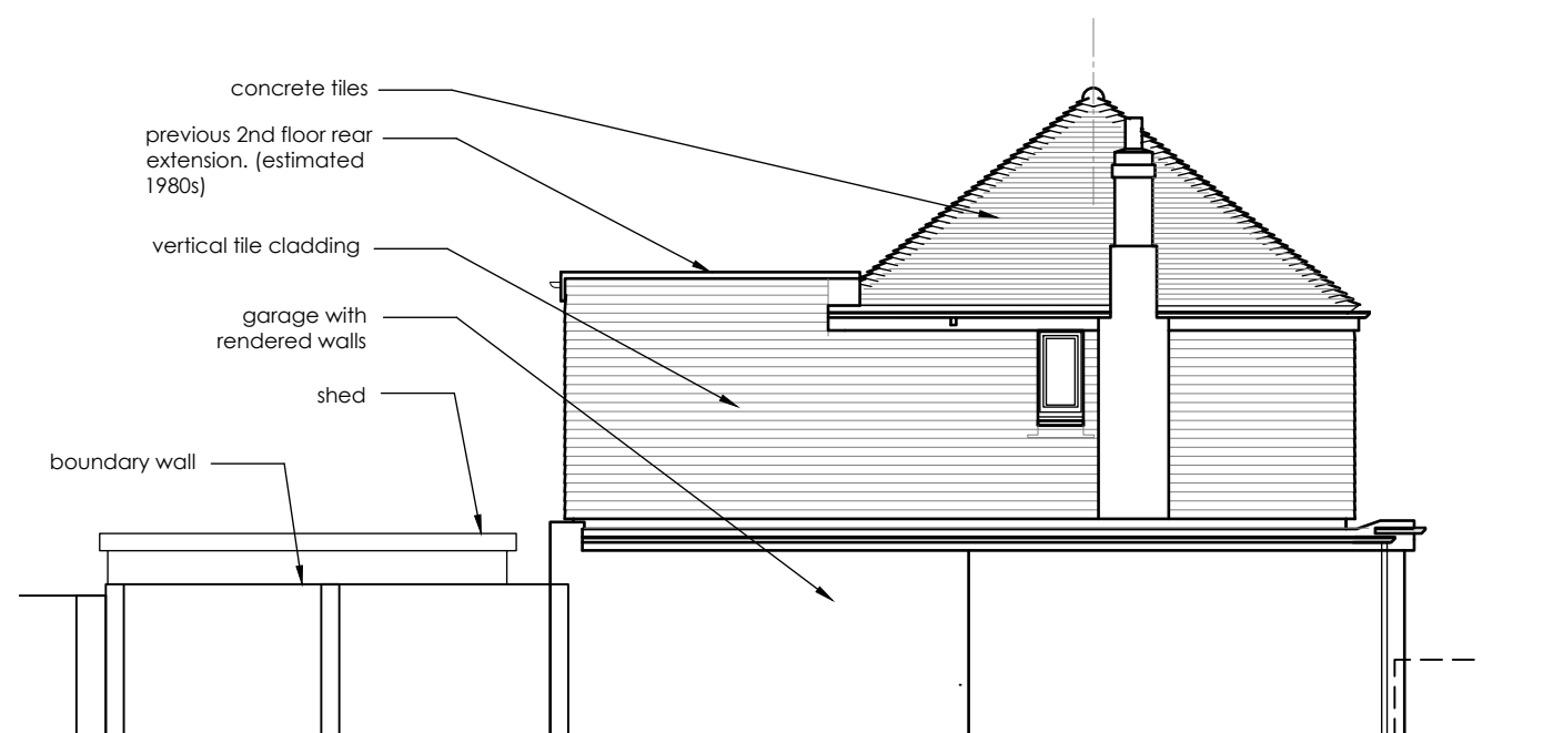
Existing West Facing Elevation (side facing no. 11)
