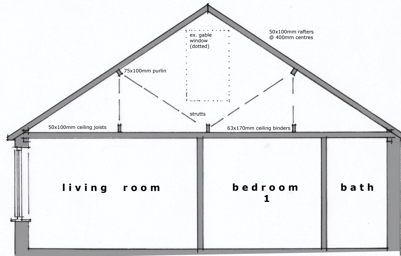
SECTION 1:50
