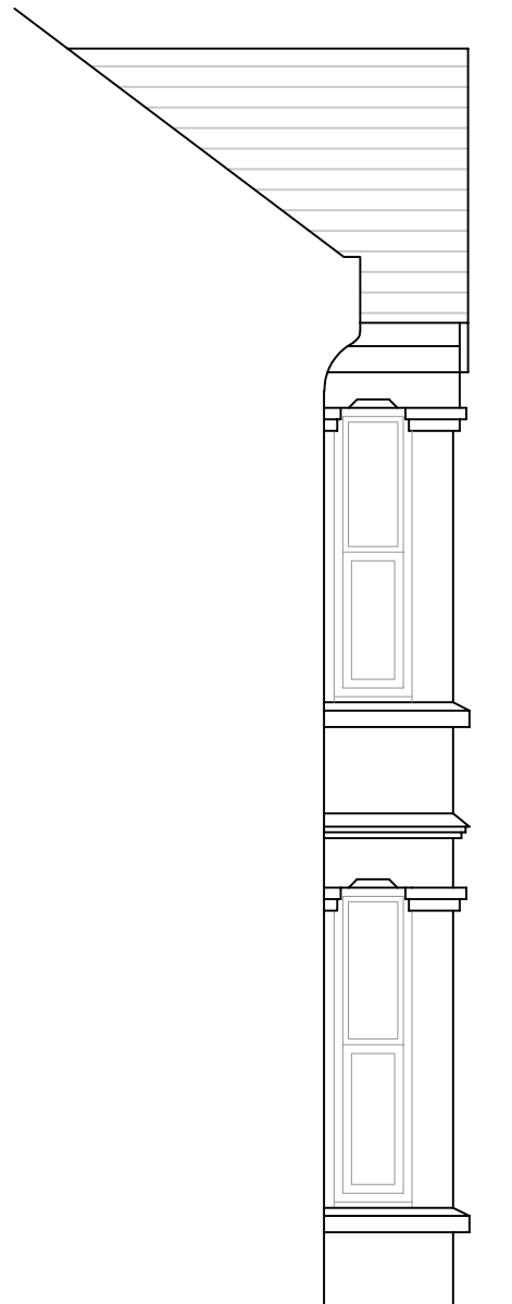
LEFT-HAND SIDE ELEVATION
