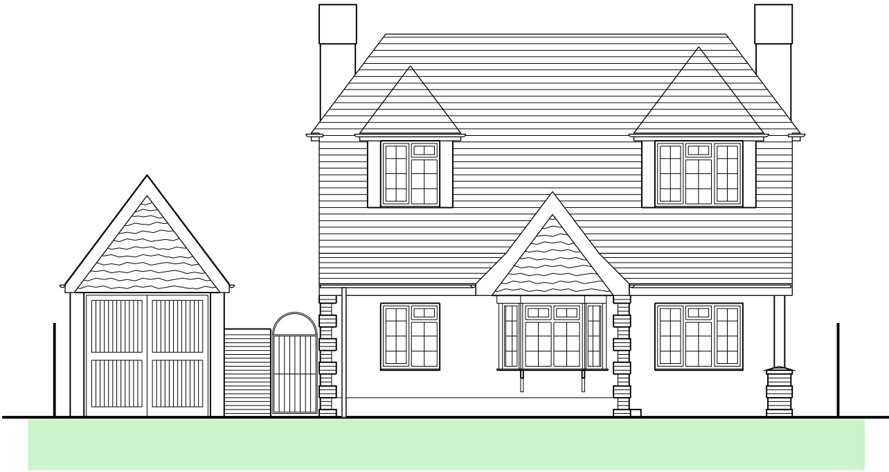
Western Elevation
