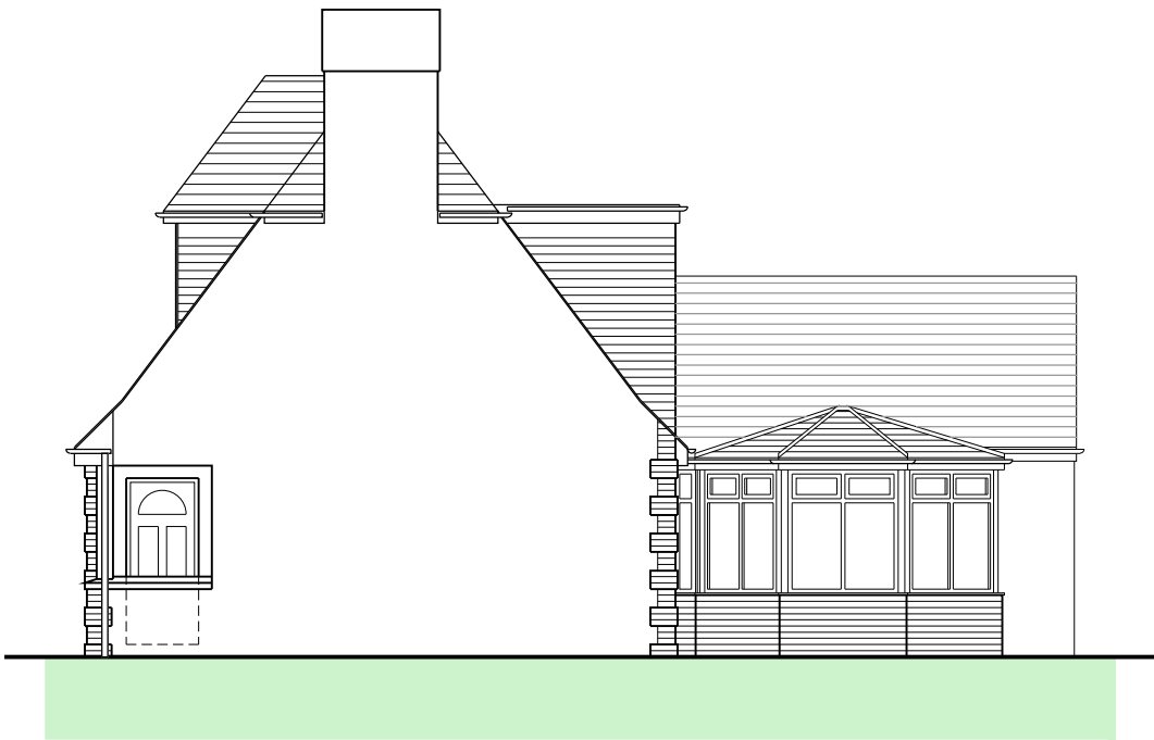
Southern Elevation
