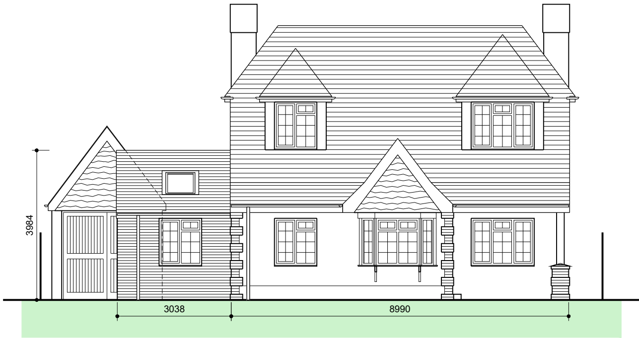
Western Elevation
