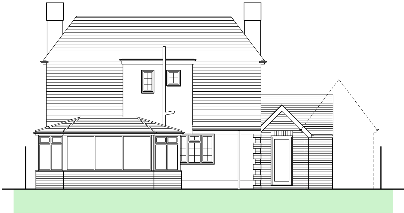
Eastern Elevation
