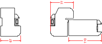
Item 1 Proposed Vertical Section Scale 1:5 @ A3
