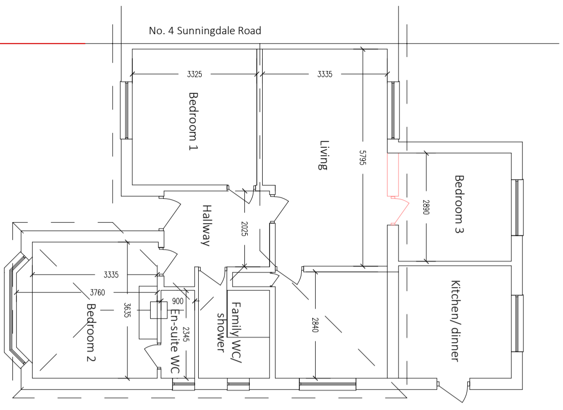
5 Existing ground floor plan
