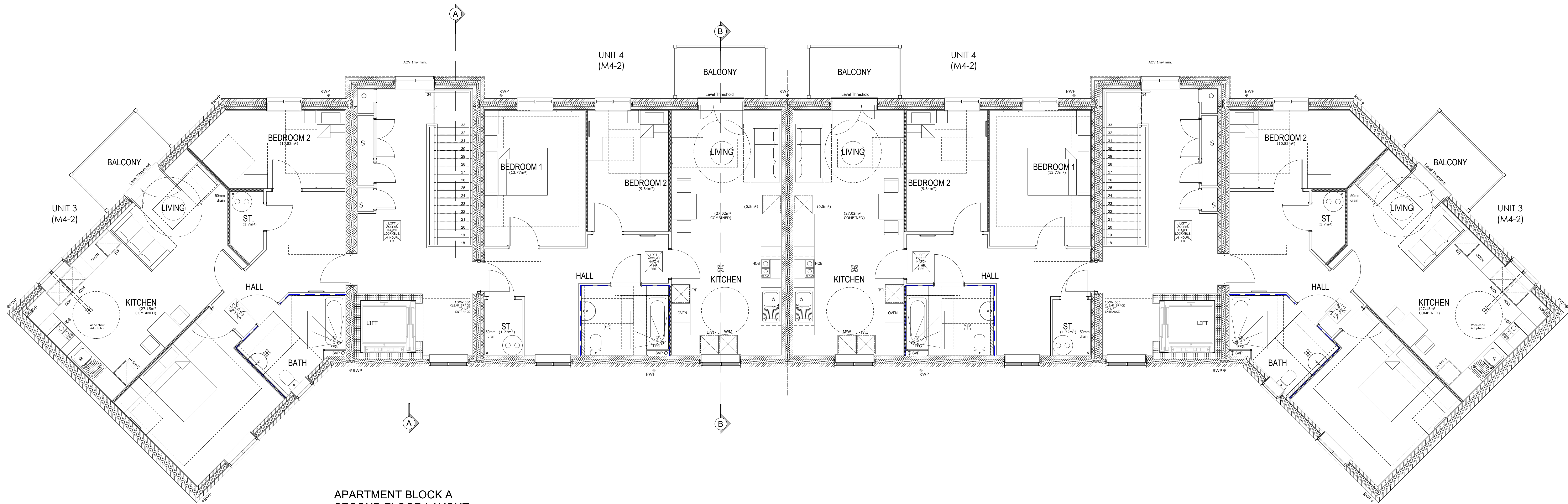
APARTMENT BLOCK A SECOND FLOOR LAYOUT
