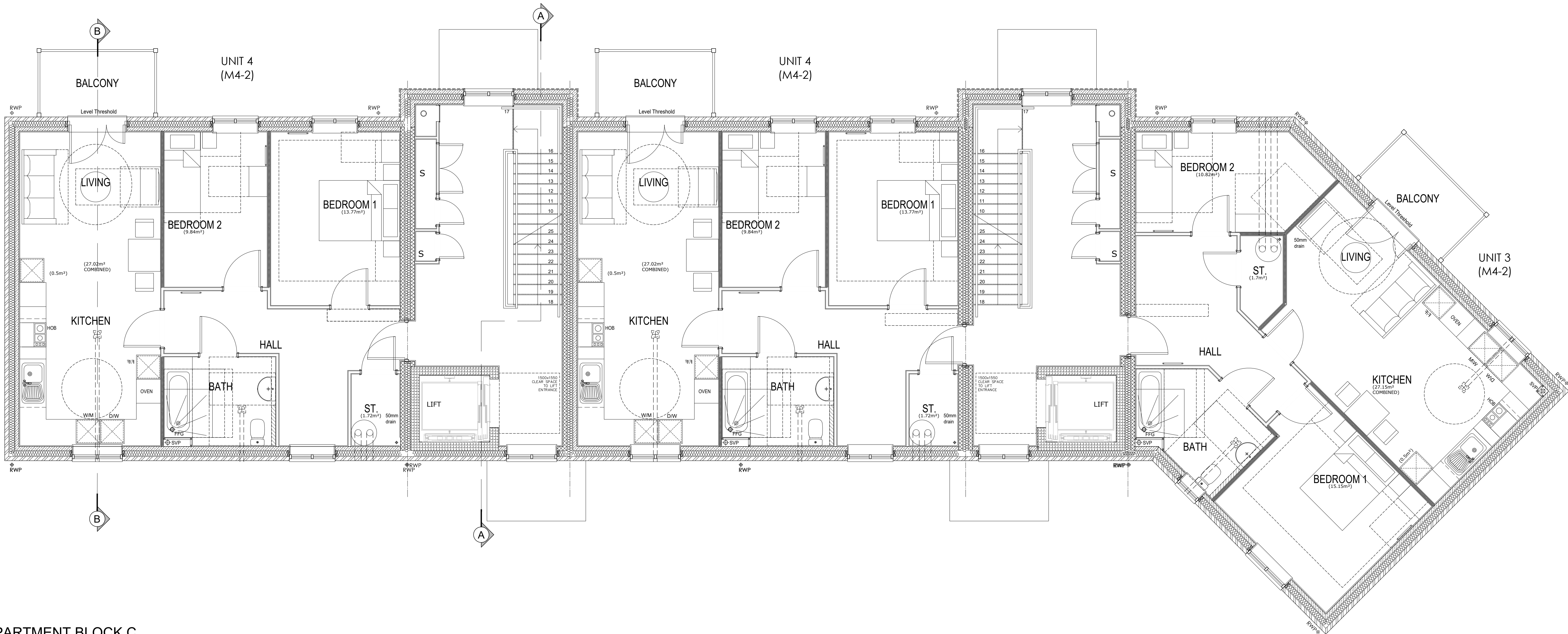
APARTMENT BLOCK C FIRST FLOOR LAYOUT
