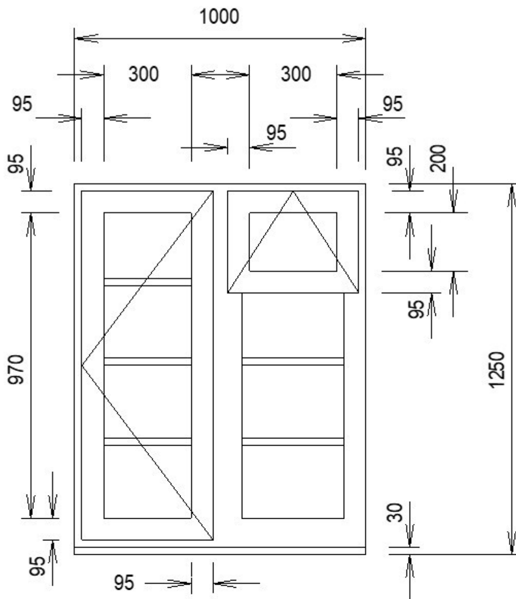
KITCHEN WINDOW with diffused MINSTER design glass
