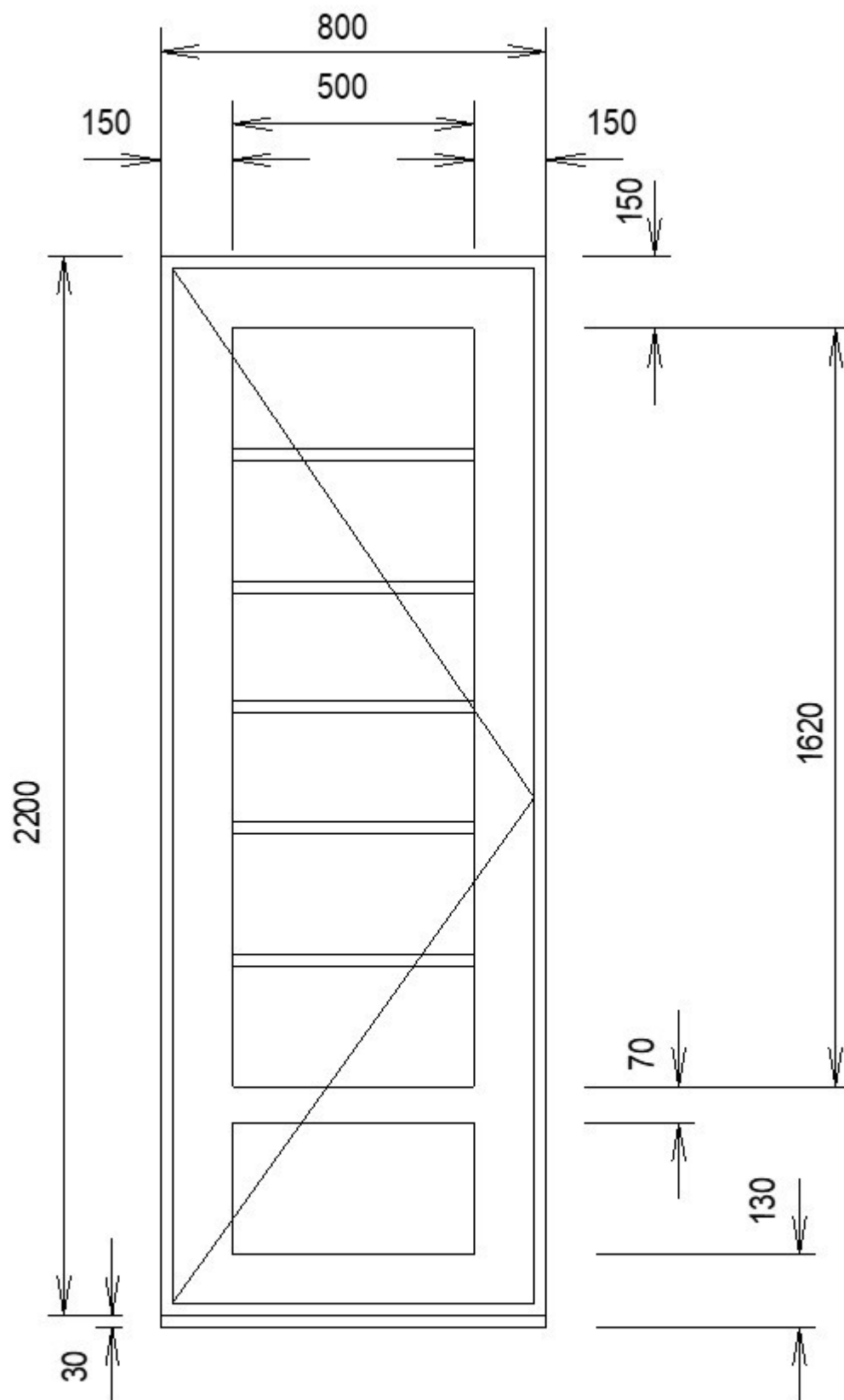
6 ARUNDEL COURT - BALCONY DOOR - AMENDED 20.01.2026 All measurements shown are in millimetres (mm)
