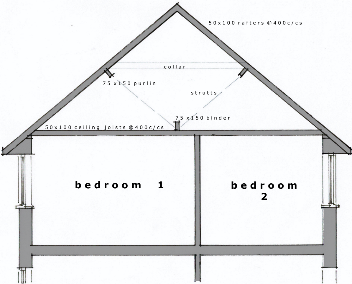
SECTION 1:50
