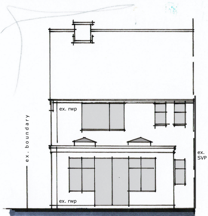
REAR (n)
