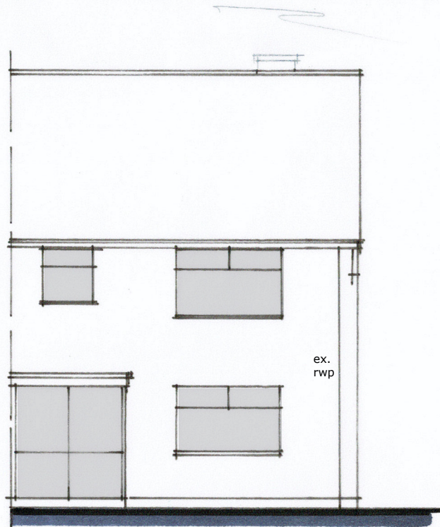
FRONT (s)
