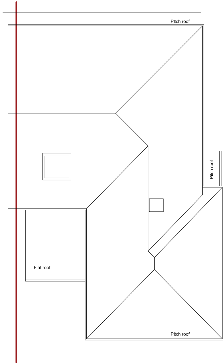
ROOF PLAN
