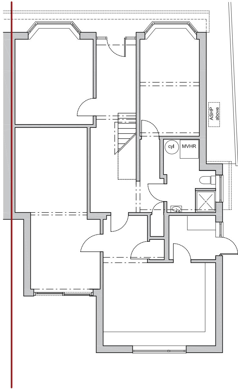
GROUND FLOOR PLAN ASHHP - Air Source Heat Pump
