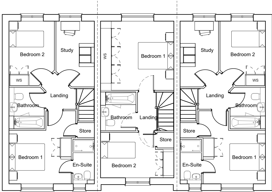
FIRST FLOOR
