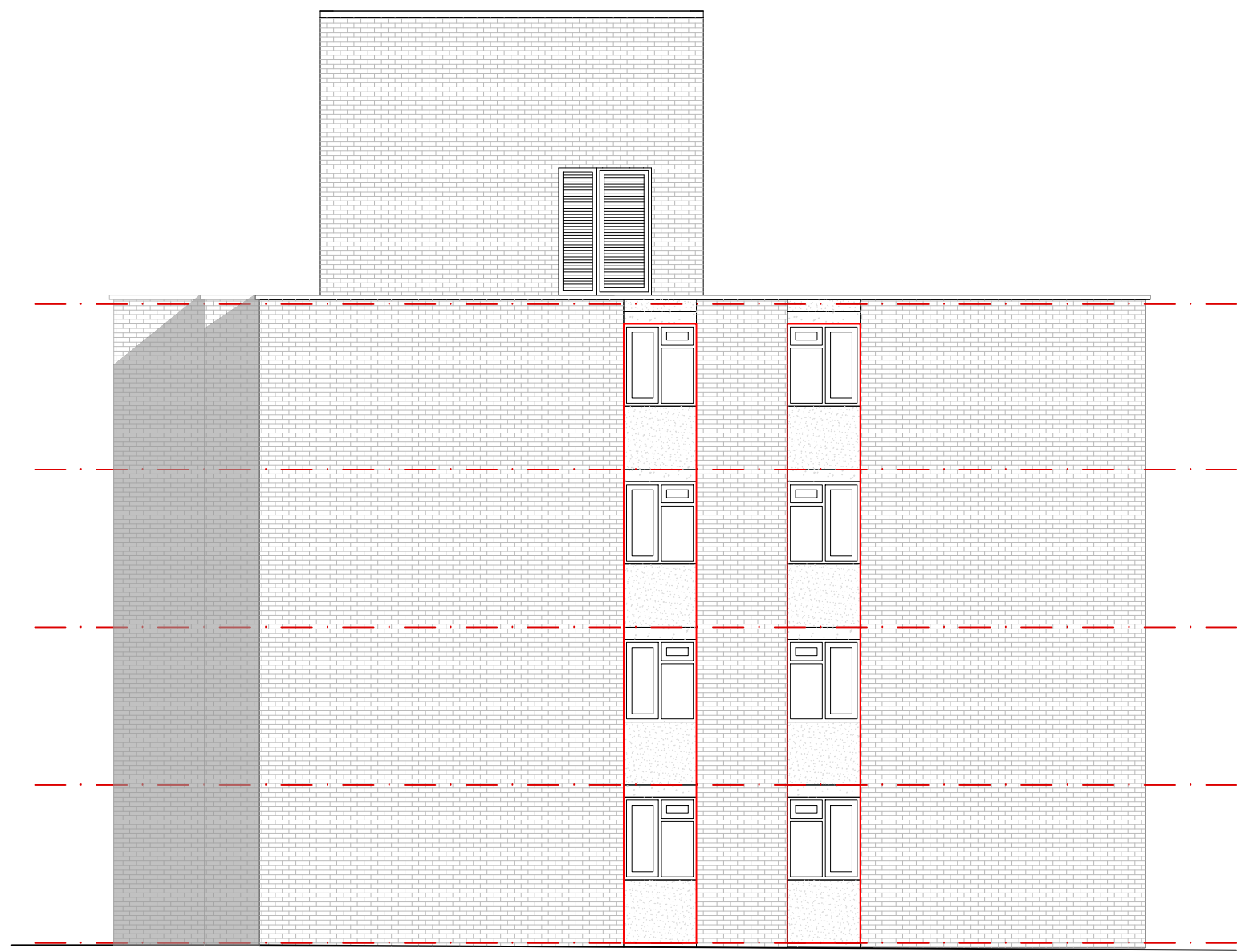
BLOCK B - (18 - 41) North Elevation
