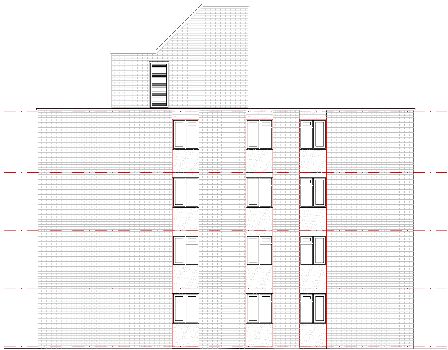
BLOCK A - (1 - 17) North Elevation
