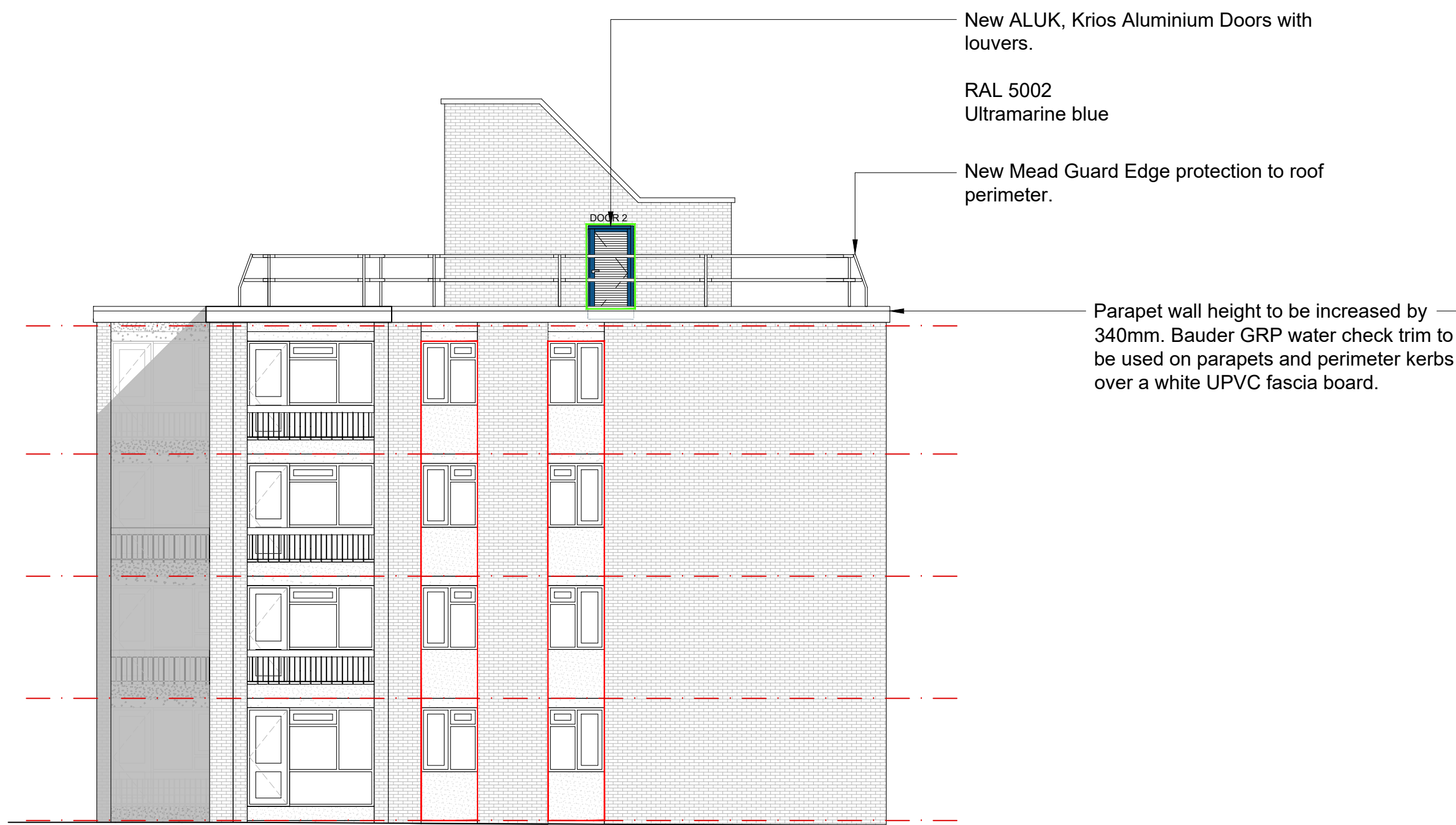
BLOCK A - (1 - 17) South Elevation
