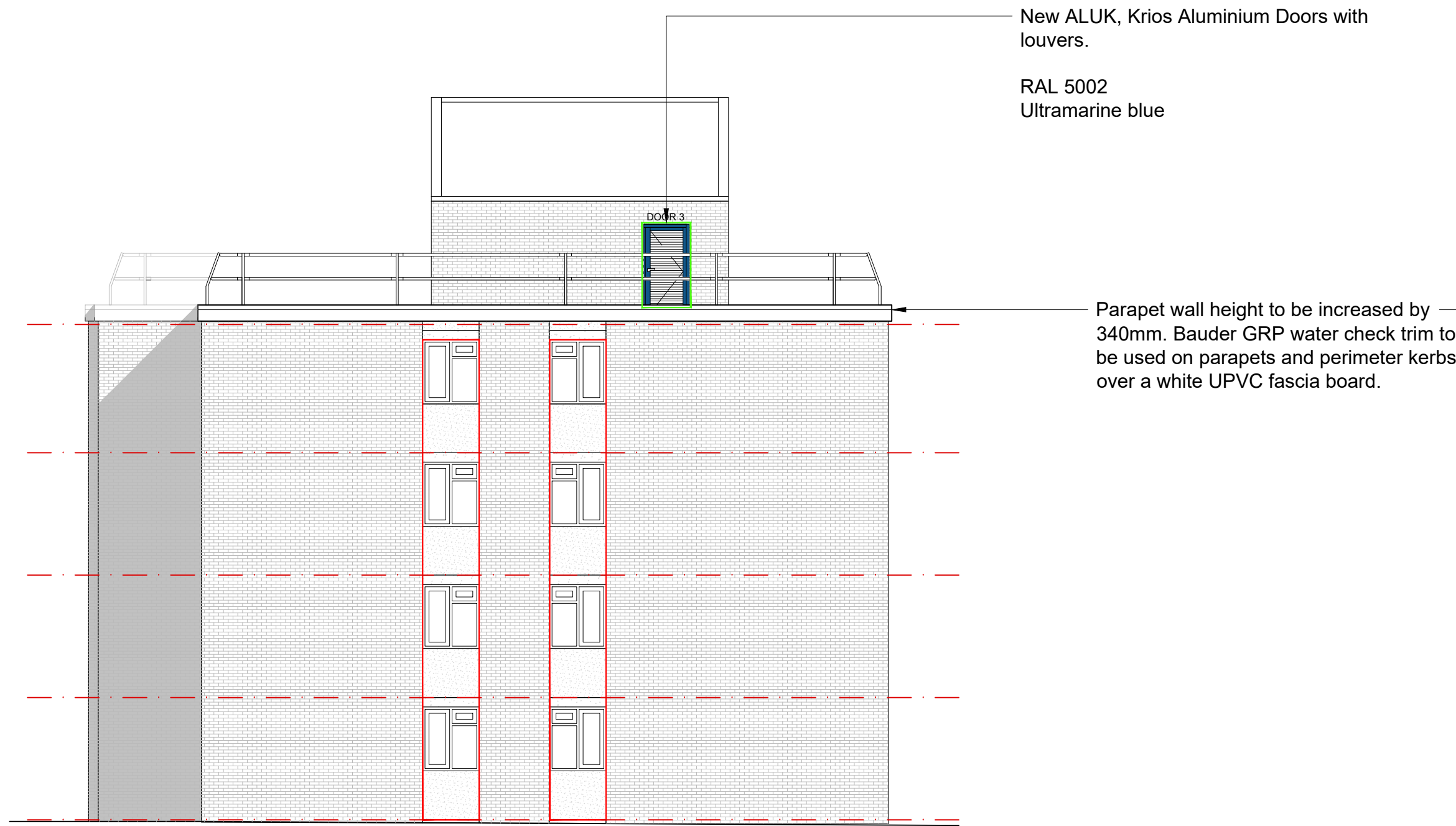
BLOCK B - (18 - 41) South Elevation
