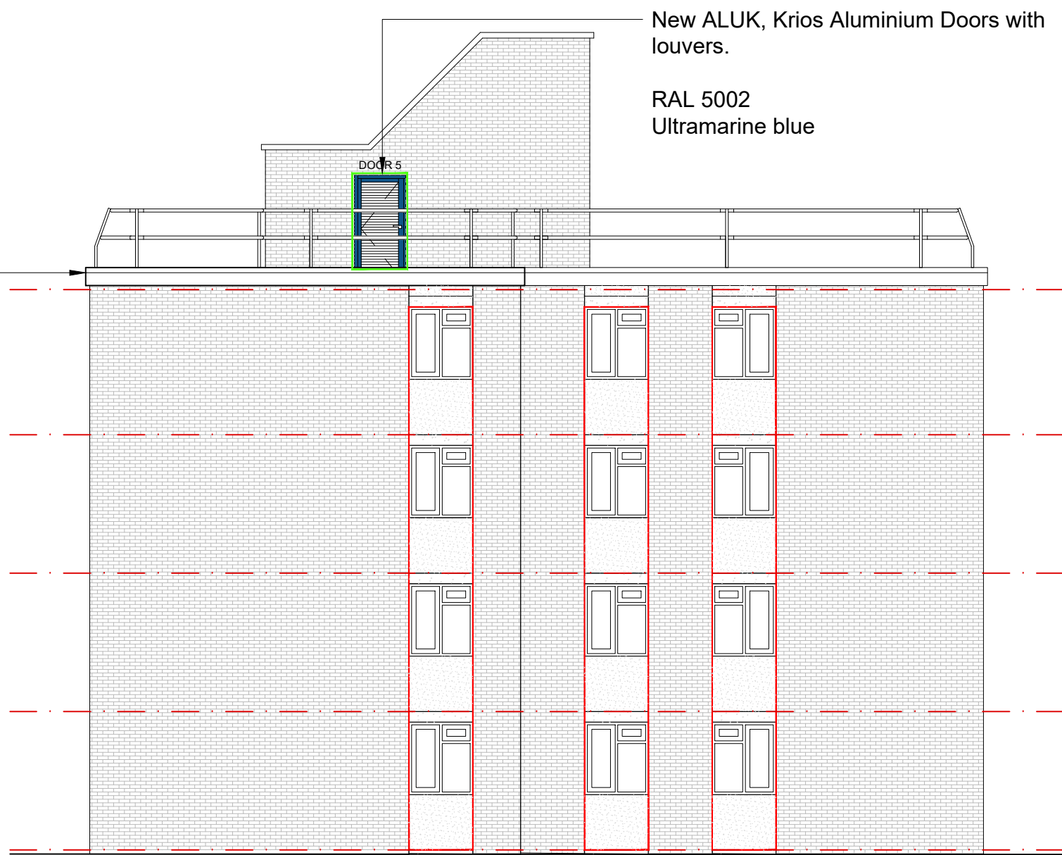
BLOCK A - (1 - 17) North Elevation
