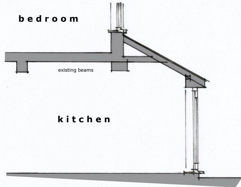
SECTION 1:50
