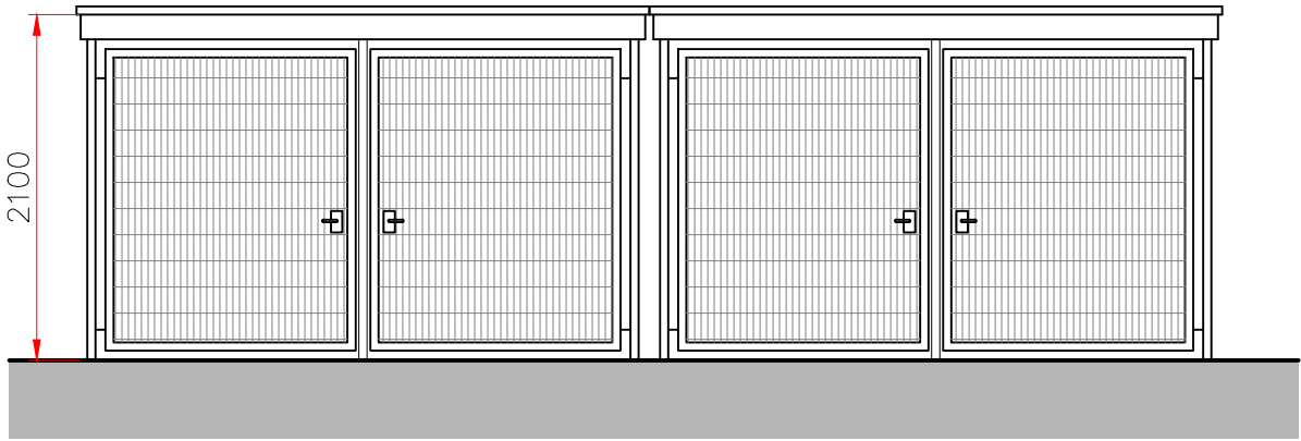
FRONT ELEVATION
