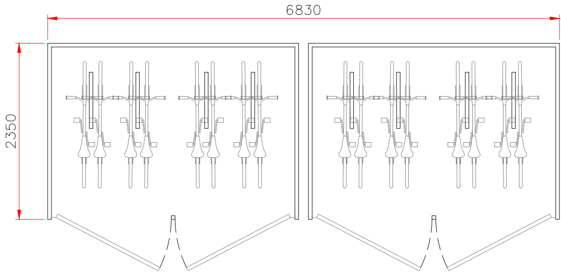
PLAN - 16no. bicycles
