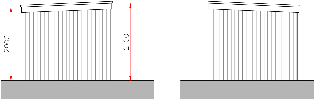
SIDE ELEVATIONS
