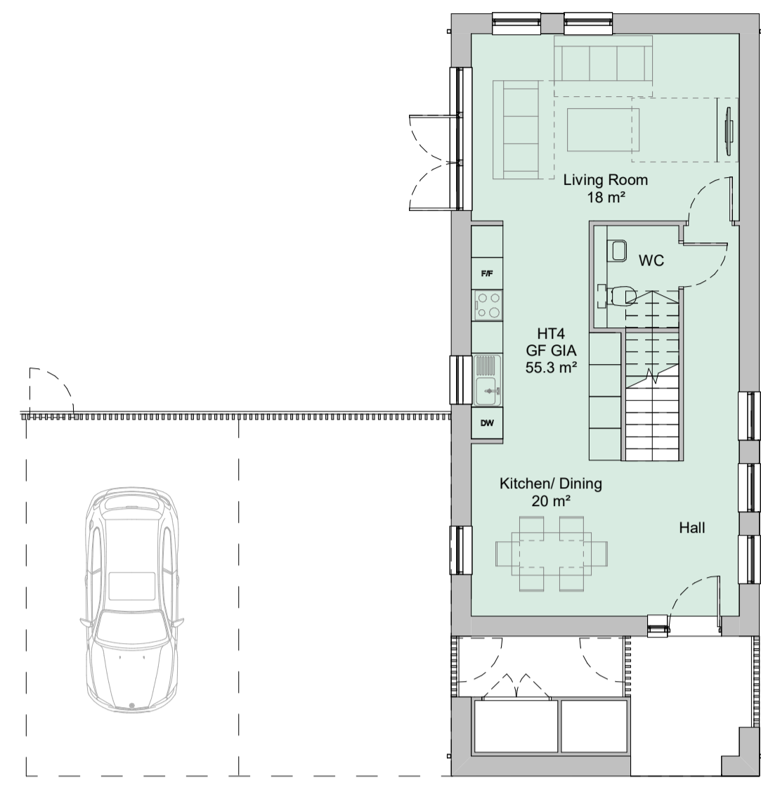
00 Ground Floor Plan 1 : 100
