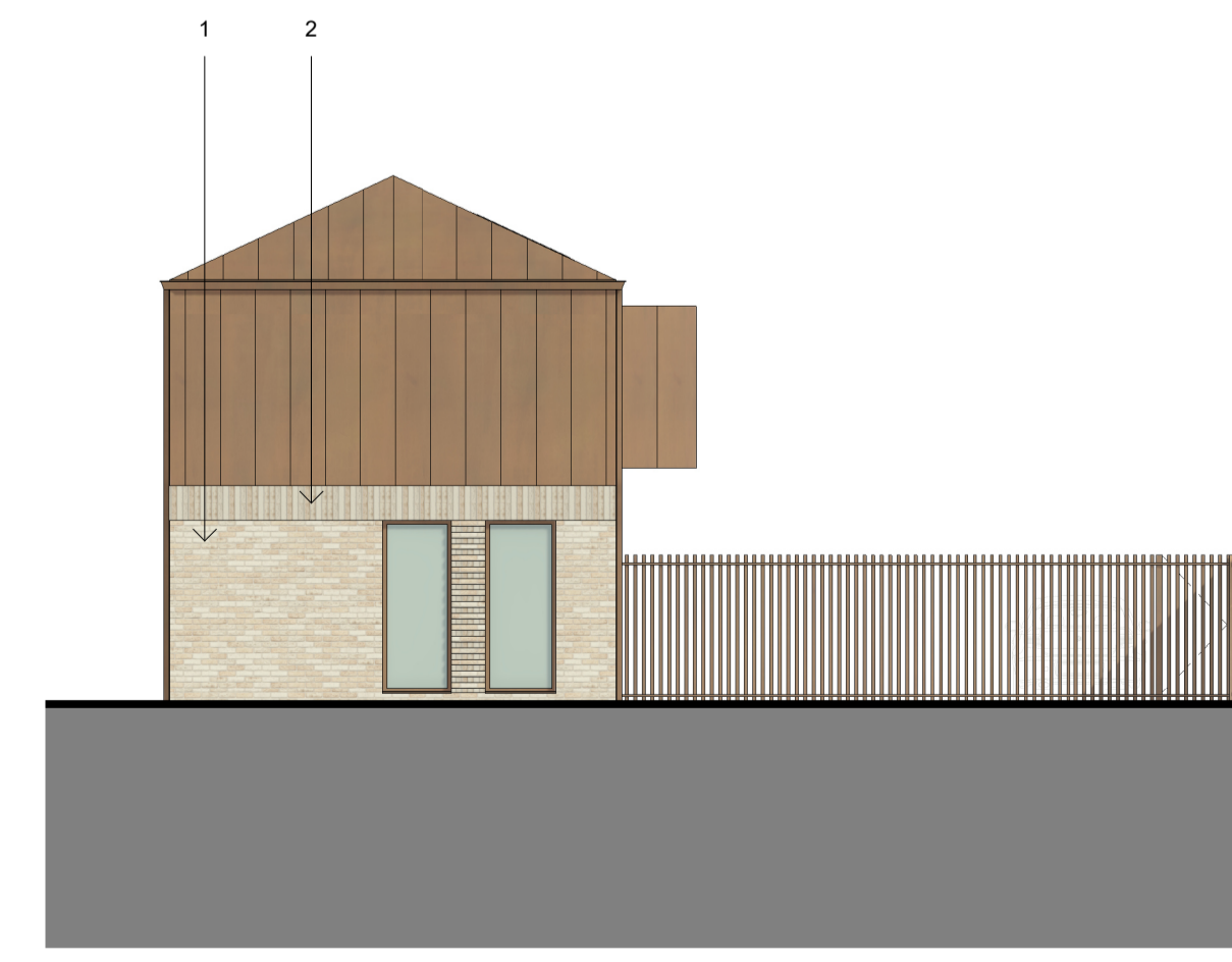
Rear Elevation 1 : 100
