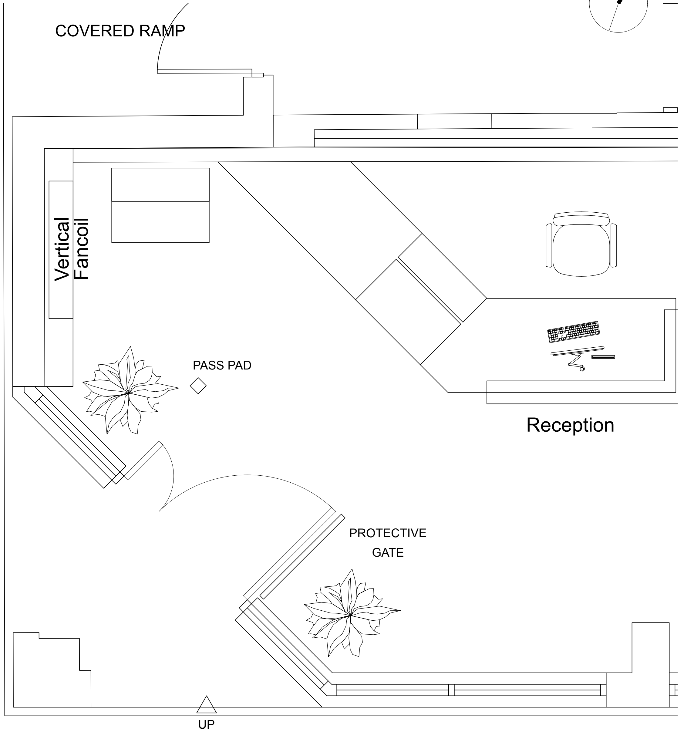
02 Detailed Area of Floor Plan 1:20 @ A1
