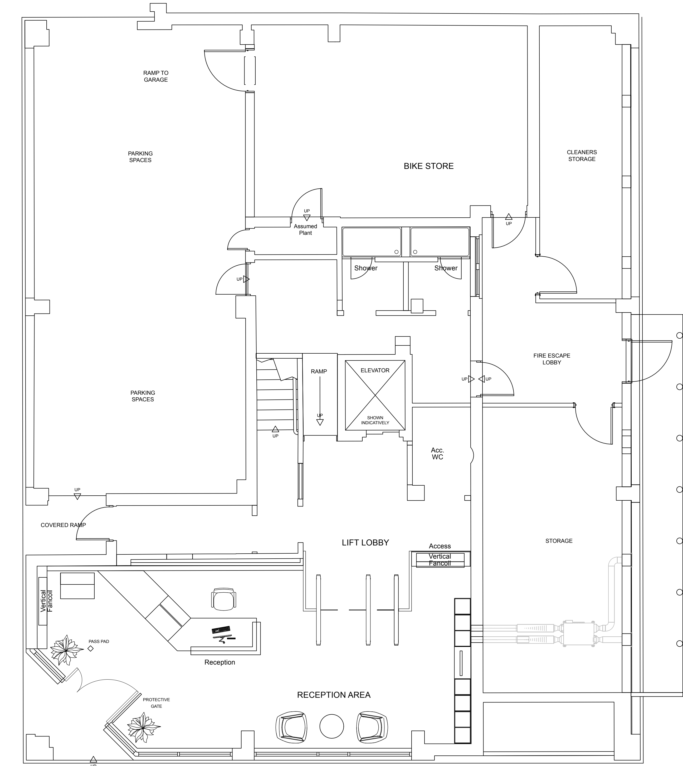
01 Floor Plan 1:50 @ A1
