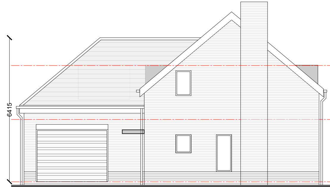
SIDE ELEVATION C
