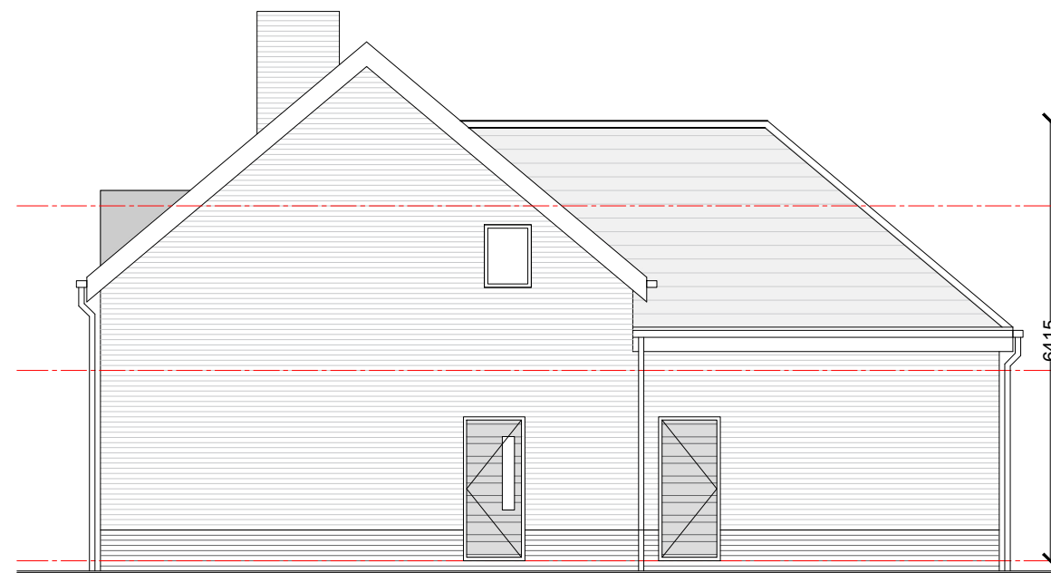
SIDE ELEVATION A
