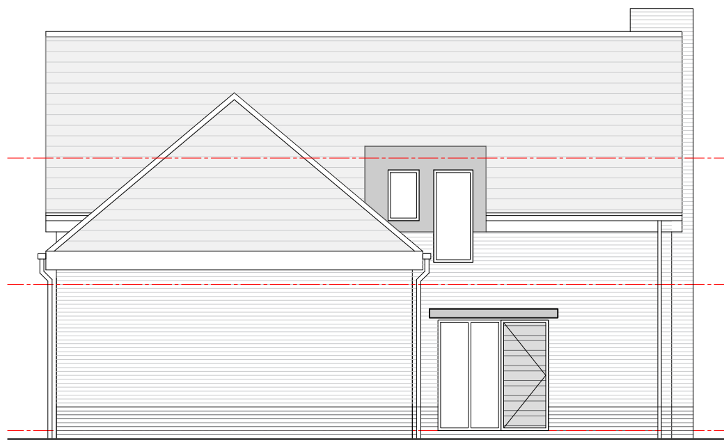
FRONT ELEVATION D
