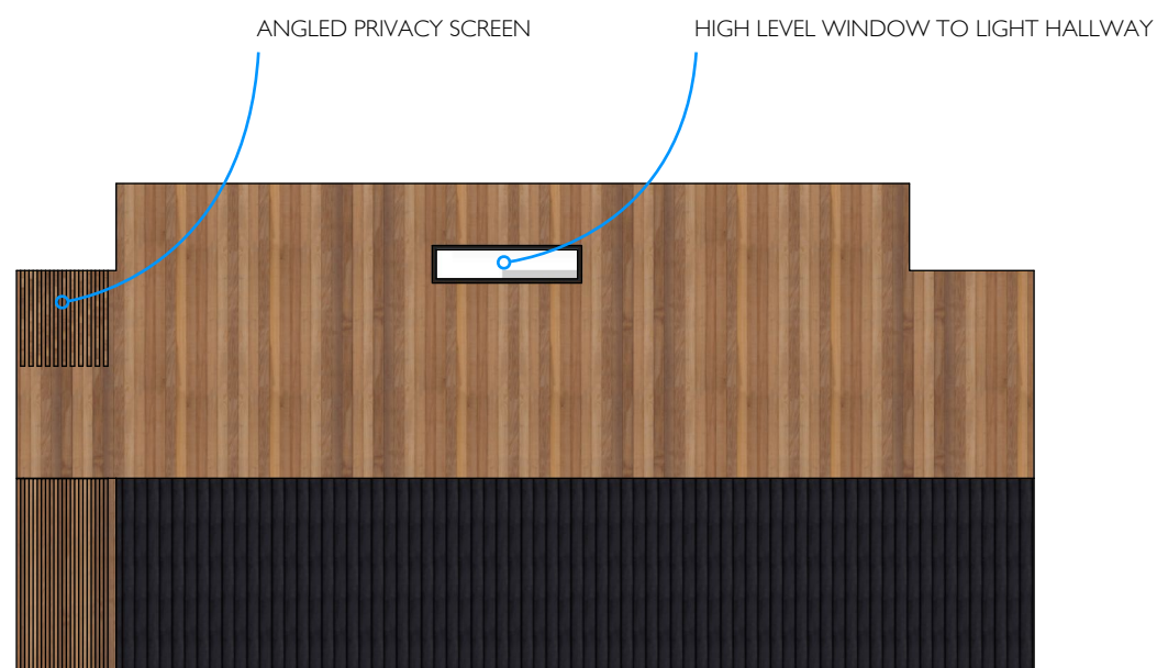
NORTHERN ELEVATION
