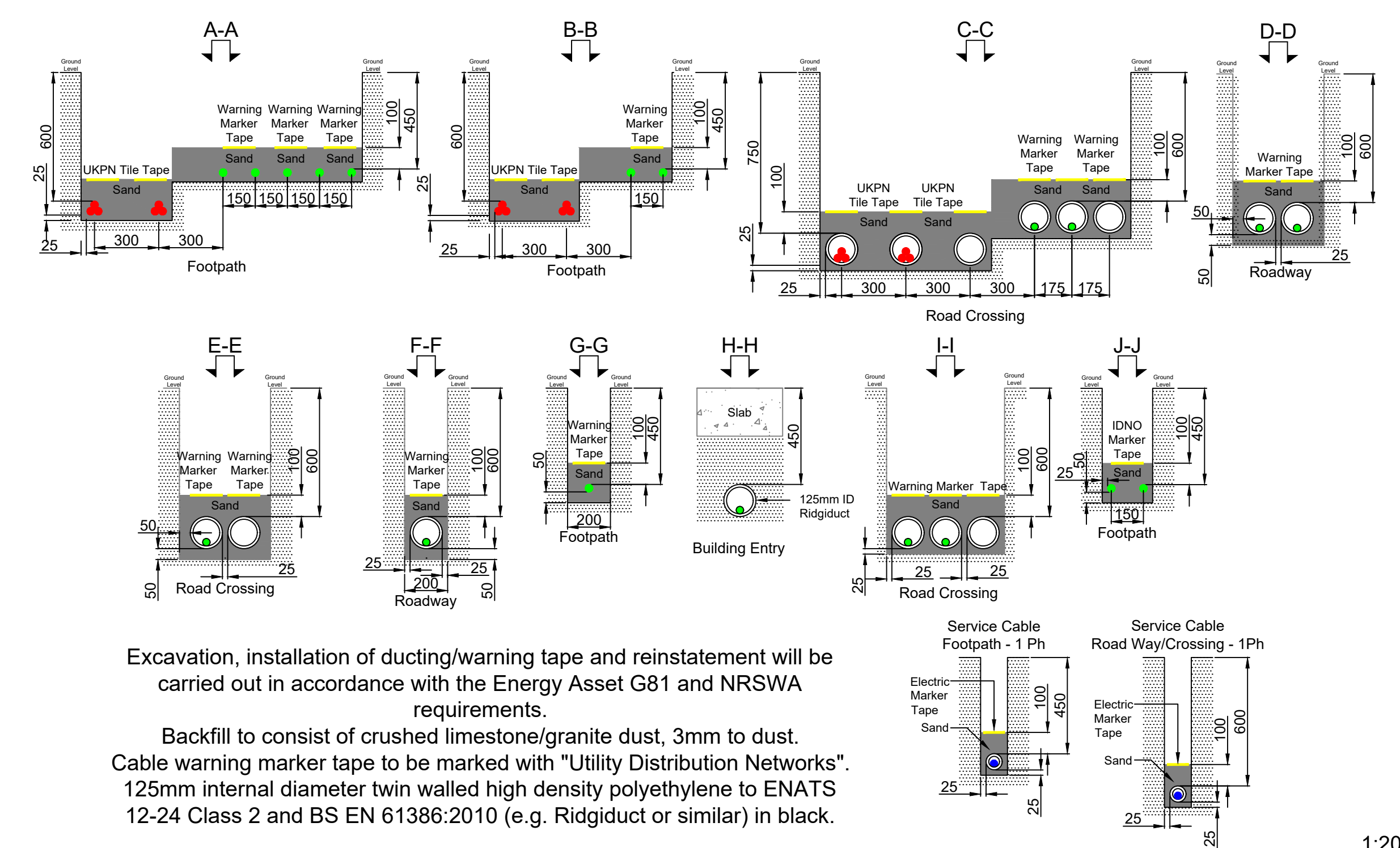
IDNO Trench Cross Sections
