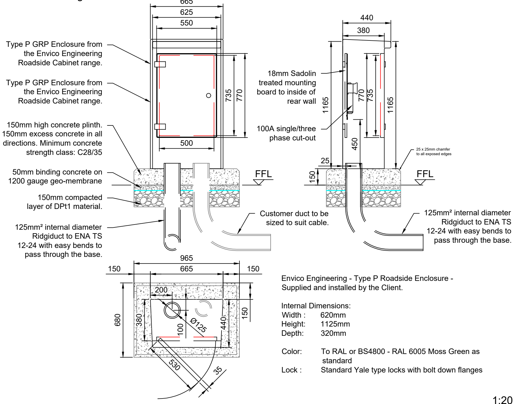
External Metering Detail
