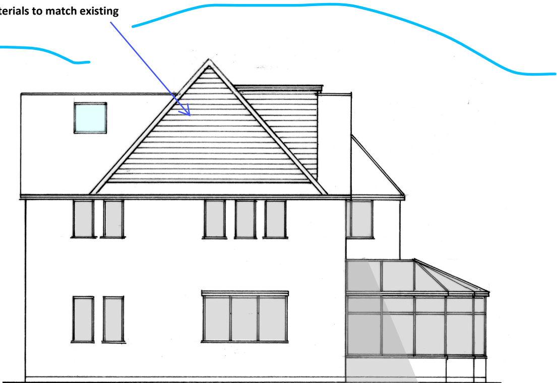
Proposed Side Elevation (South) 1:100
