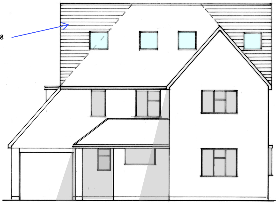
Proposed Front Elevation (West) 1:100
