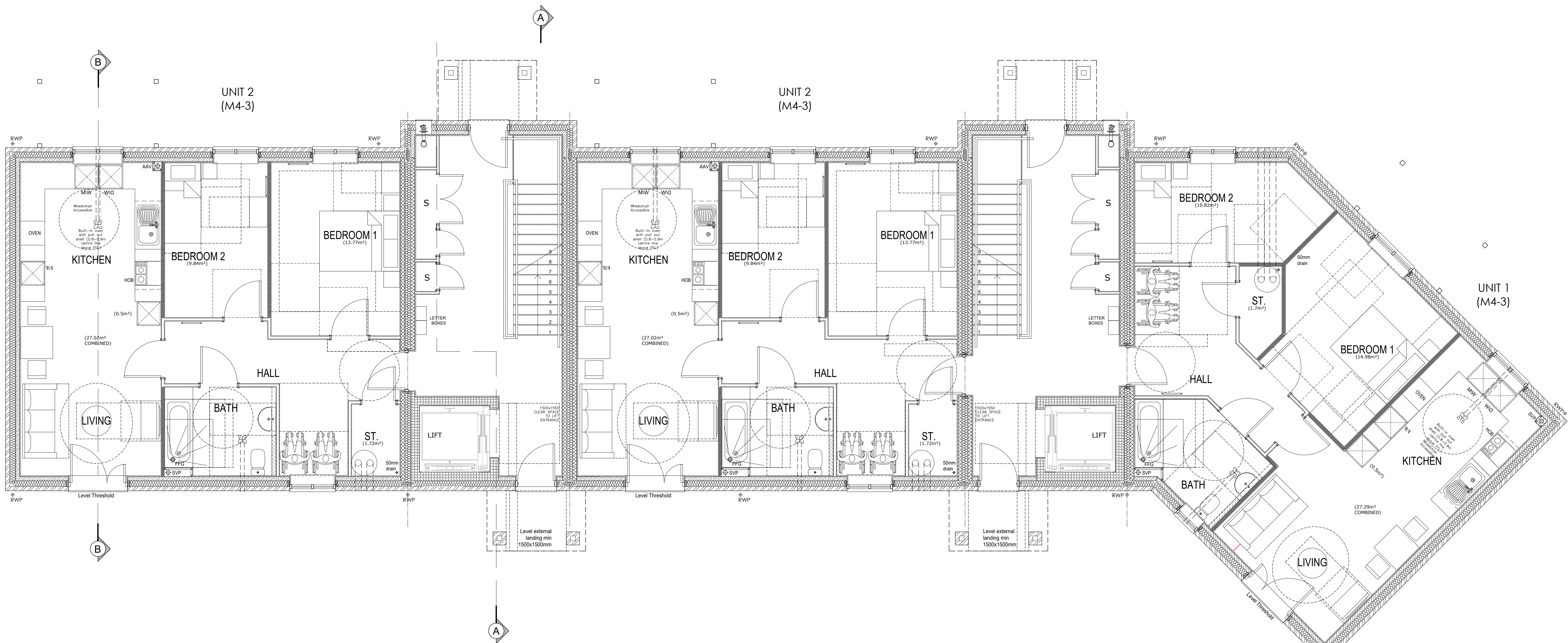
APARTMENT BLOCK C GROUND FLOOR LAYOUT PLOTS 174 - 182
