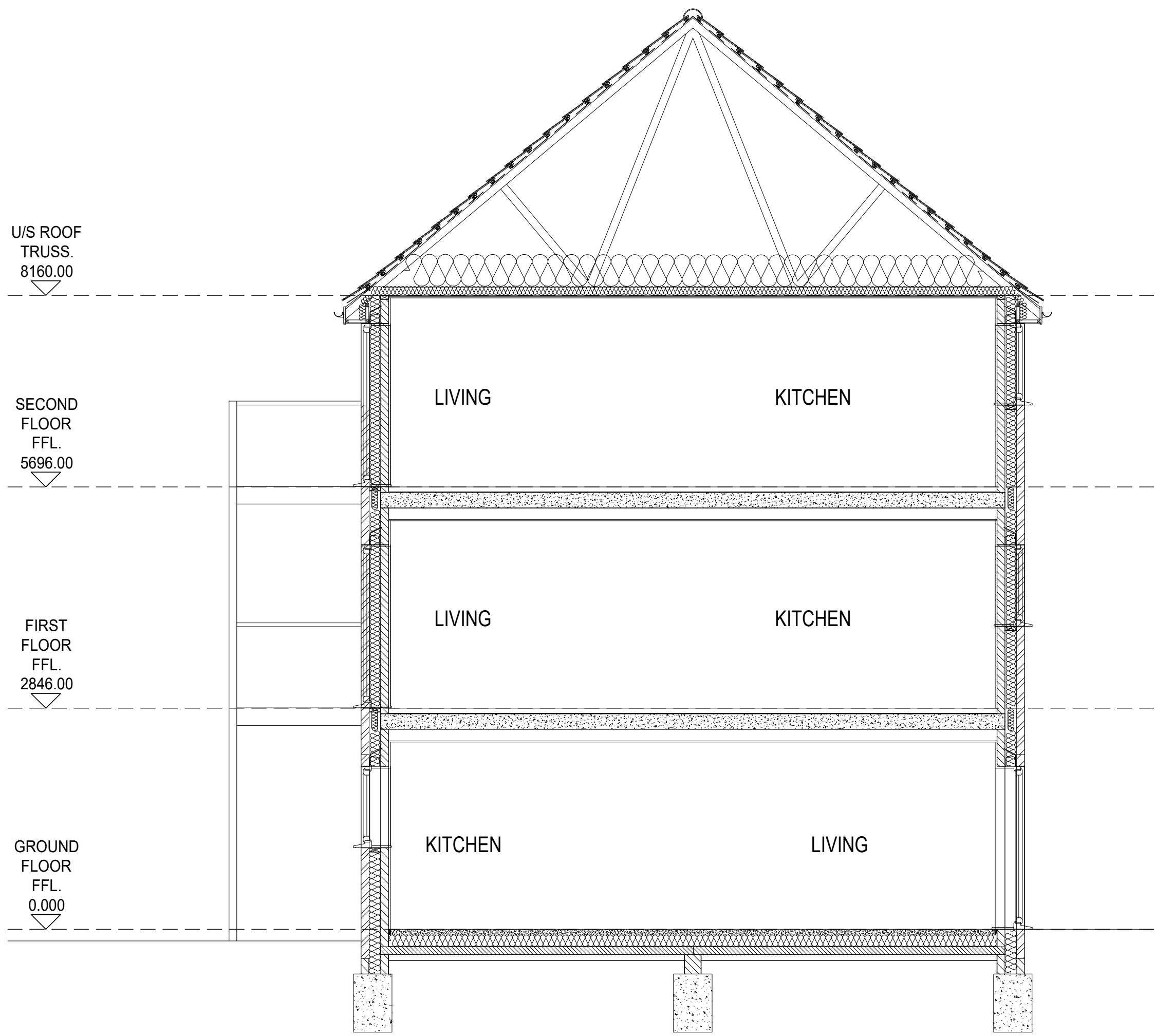
SECTION B-B
