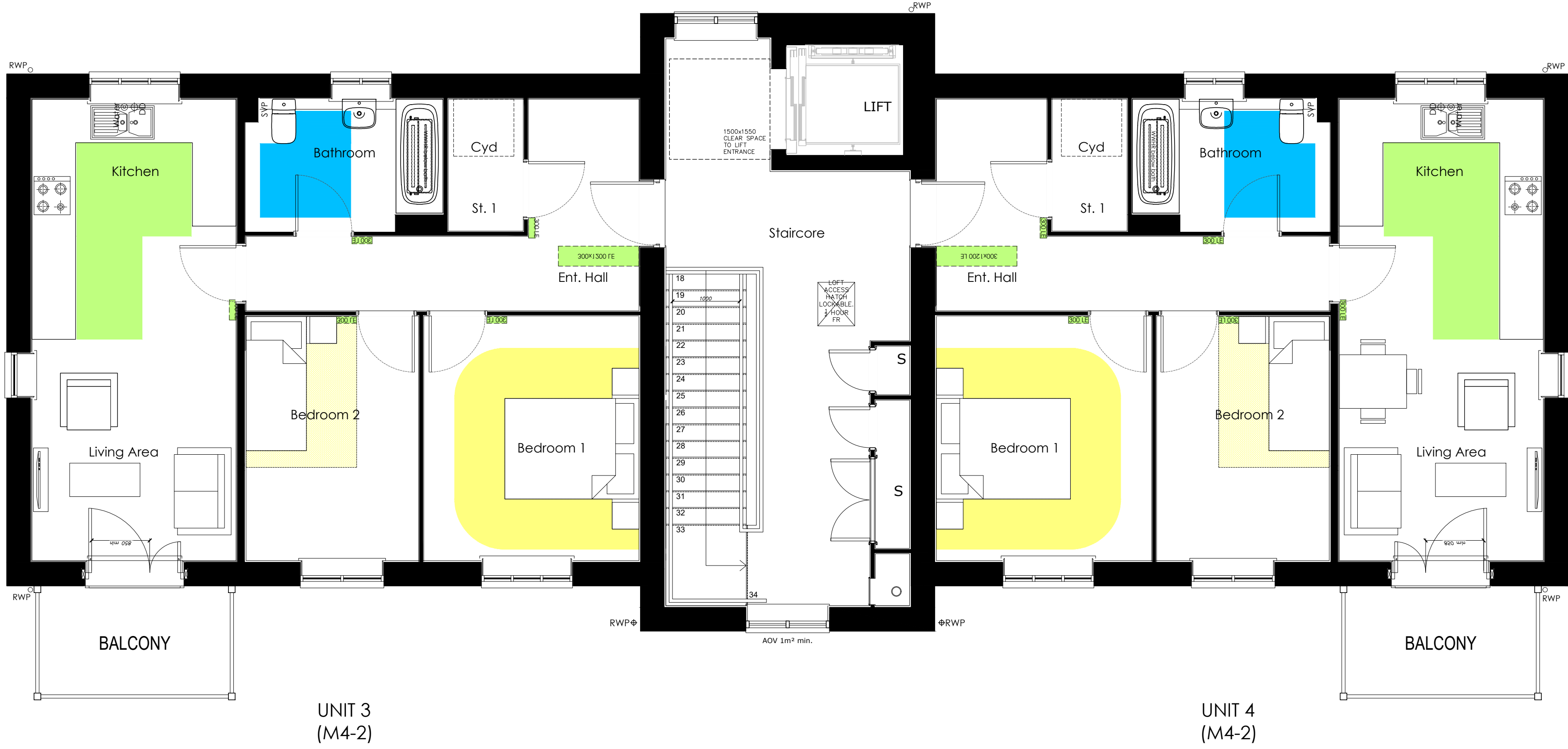
APARTMENT BLOCK D SECOND FLOOR LAYOUT
