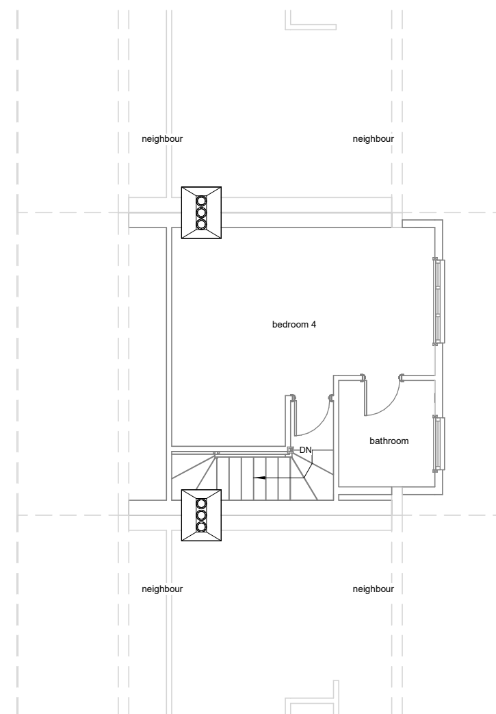
Proposed Loft Floor
