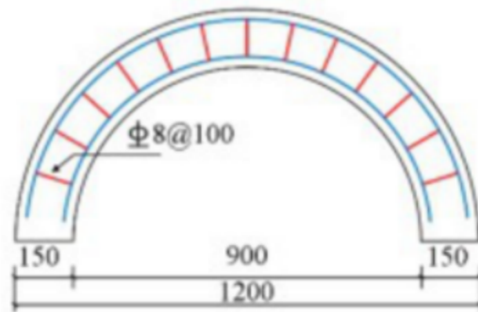
Reinforcement Drawing (Unit: mm)
