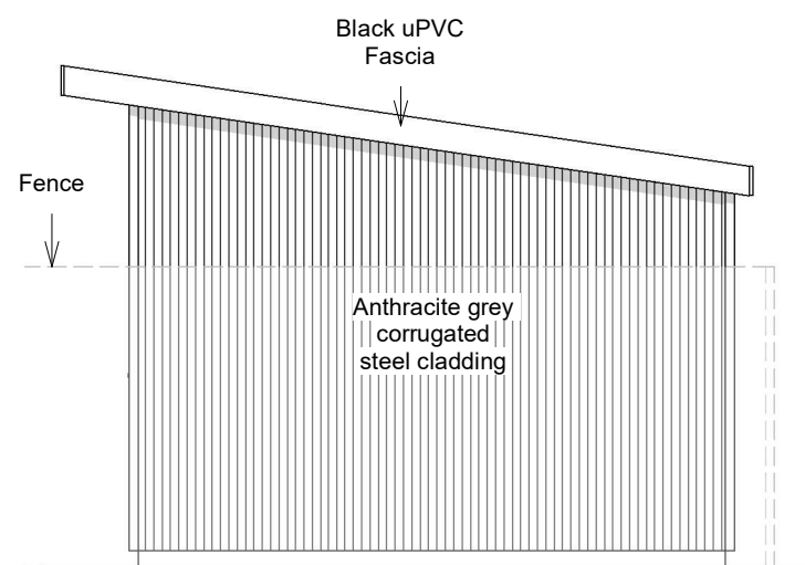
South Elevation
