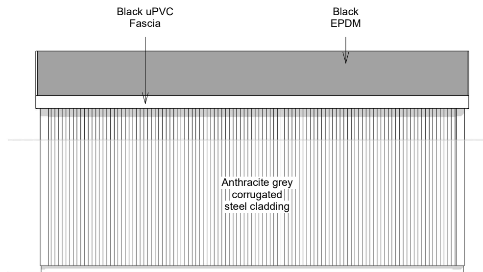
East Elevation
