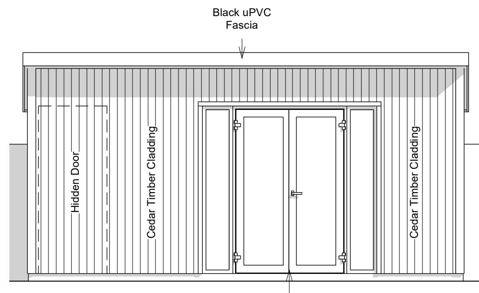
West Elevation
