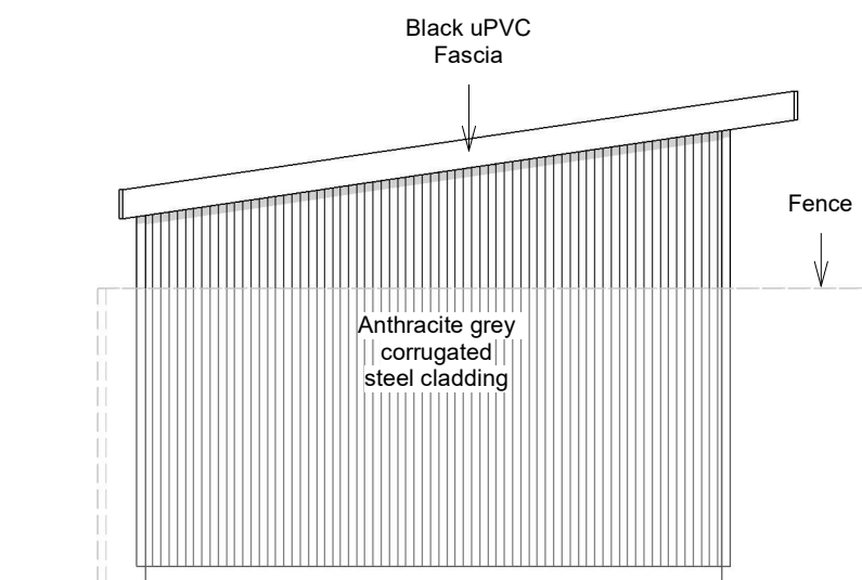
North Elevation
